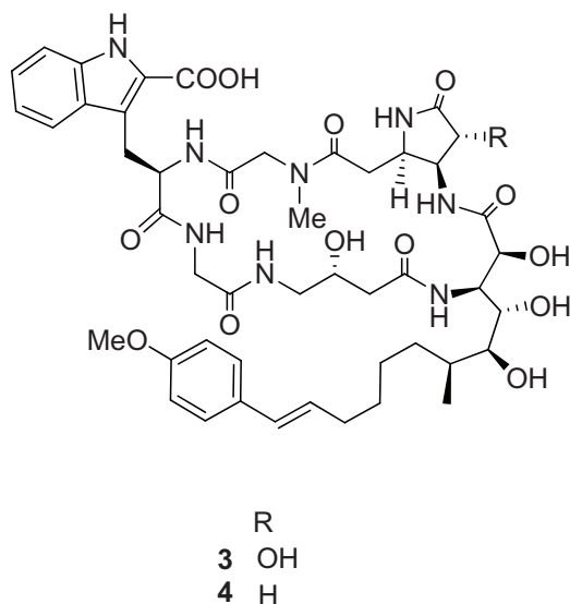
Figure 1 Structures of compounds 1 – 4 .
