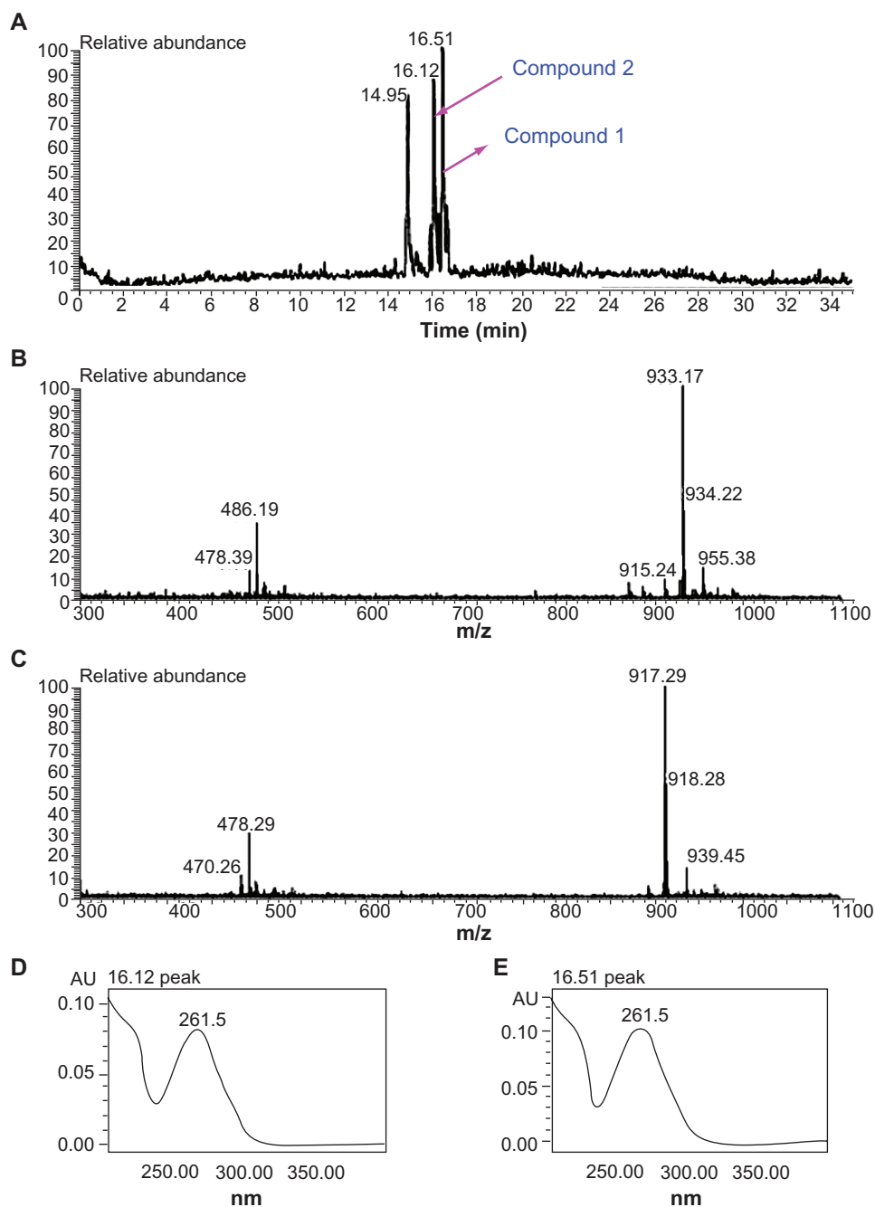
Figure 2 LC-MS analysis of antifungal column fraction D: (A) base peak chromatogram (BPC); (B) positive ESIMS spectrum for the peak with a retention time of 16.12 minutes, corresponding to compound 2 ; (C) positive ESIMS spectrum for the peak with a retention time of 16.51 minutes, corresponding to compound 1 ; (D) UV spectrum for the peak with a retention time of 16.12 minutes, corresponding to compound 2 ; and (E) UV spectrum for the peak with a retention time of 16.51 minutes, corresponding to compound 1 .
