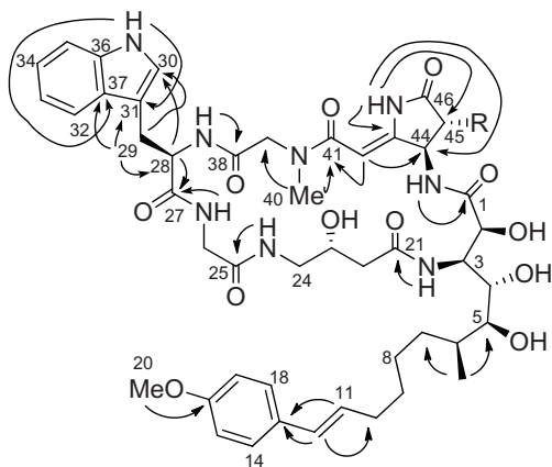
Figure 3 Key HMBC correlations for compounds 1 and 2.
