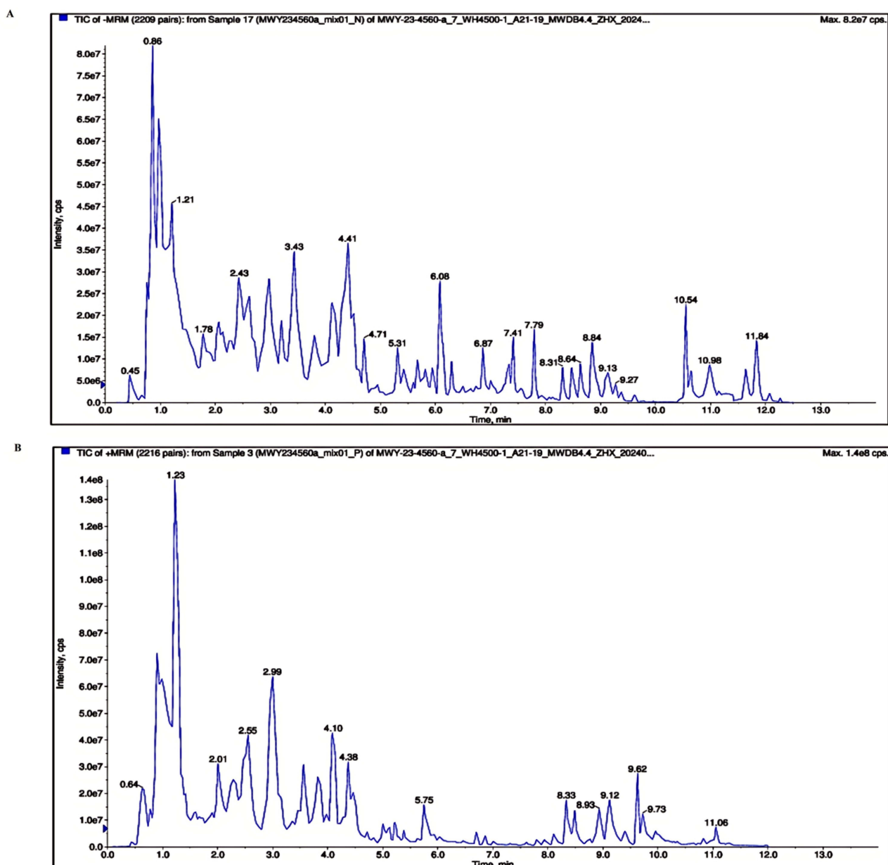
Figure 1 Total ion chromatogram (TIC) diagram of MZGW. (A) In positive ion mode. (B) In negative ion mode.
