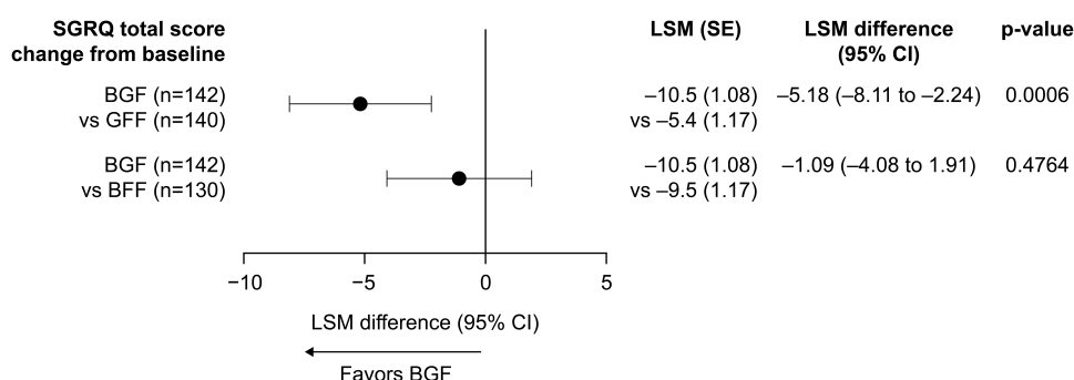
Figure 3 Change in SGRQ total score over 24 weeks in patients with COPD and phenotypic features of asthma, 3 pooled KRONOS and ETHOS mITT populations (n = 412). Note: 3 Patients from the mITT population with reversibility to salbutamol ( \geq 12\% and \geq 200 mL increase in FEV 1 after administration of salbutamol) and blood eosinophils \geq 300 cells/mm 3 .
