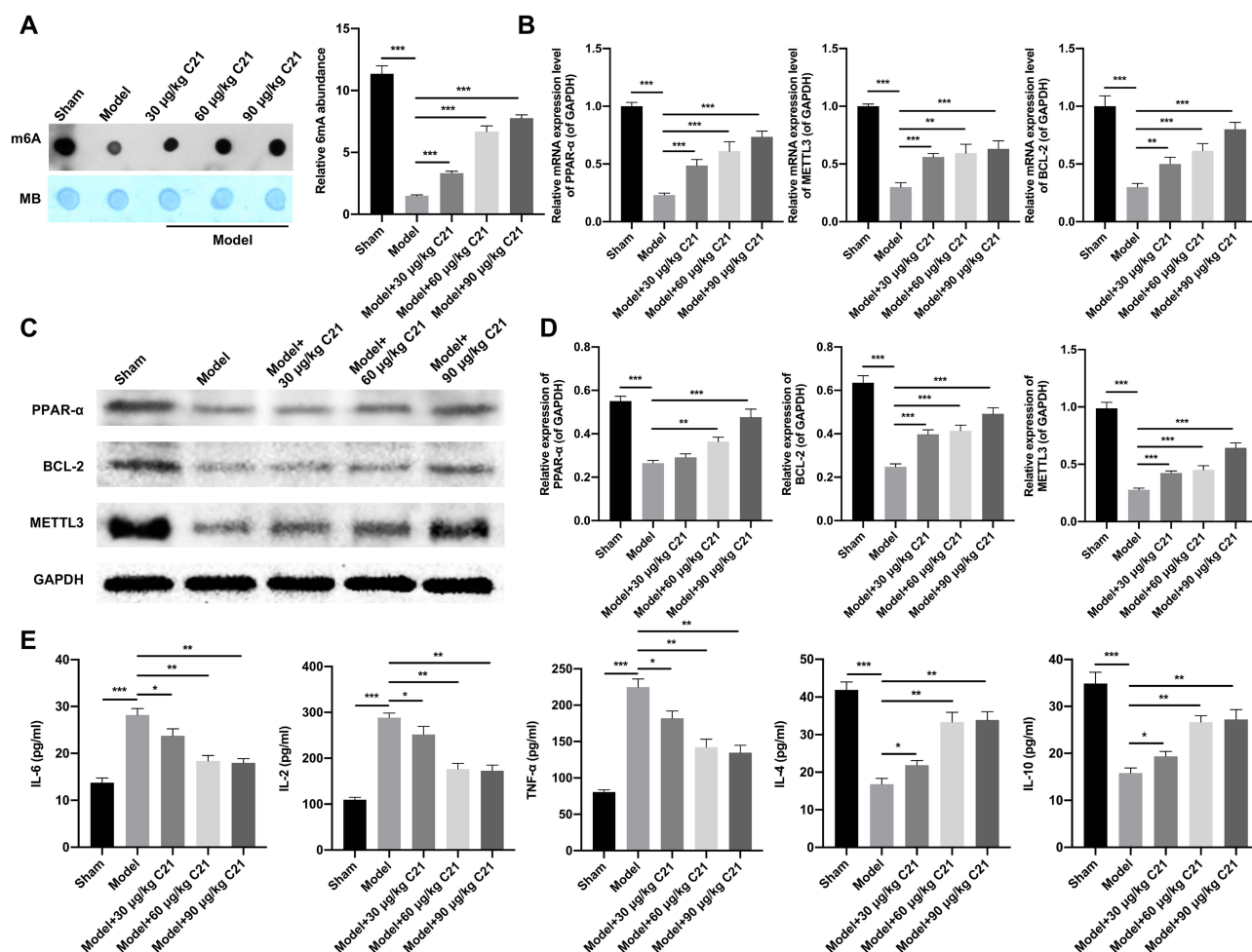
Figure 3 C21 upregulates the levels of m6A modification, PPAR- \alpha , BCL-2, and METTL3 and reduces the inflammatory response in ISO-induced neonatal rats. The ISO-induced neonatal rats were processed with 30, 60, and 90 \mu\text{g/kg} C21 by intraperitoneal injection. (A) The m6A modification level was assessed using a Dot blot. (B) The expressions of PPAR- \alpha , METTL3, and BCL-2 were monitored through RT-qPCR. (C) Western blotting analysis of PPAR- \alpha , METTL3, and BCL-2 protein expressions in the hippocampus. (D) Quantitative analysis of Western blot results. (E) ELISA kits were adopted to analyze the levels of inflammation-related factors (IL-6, IL-2, TNF- \alpha , IL-4, and IL-10). * P < 0.05 , ** P < 0.01 , *** P < 0.001 .
