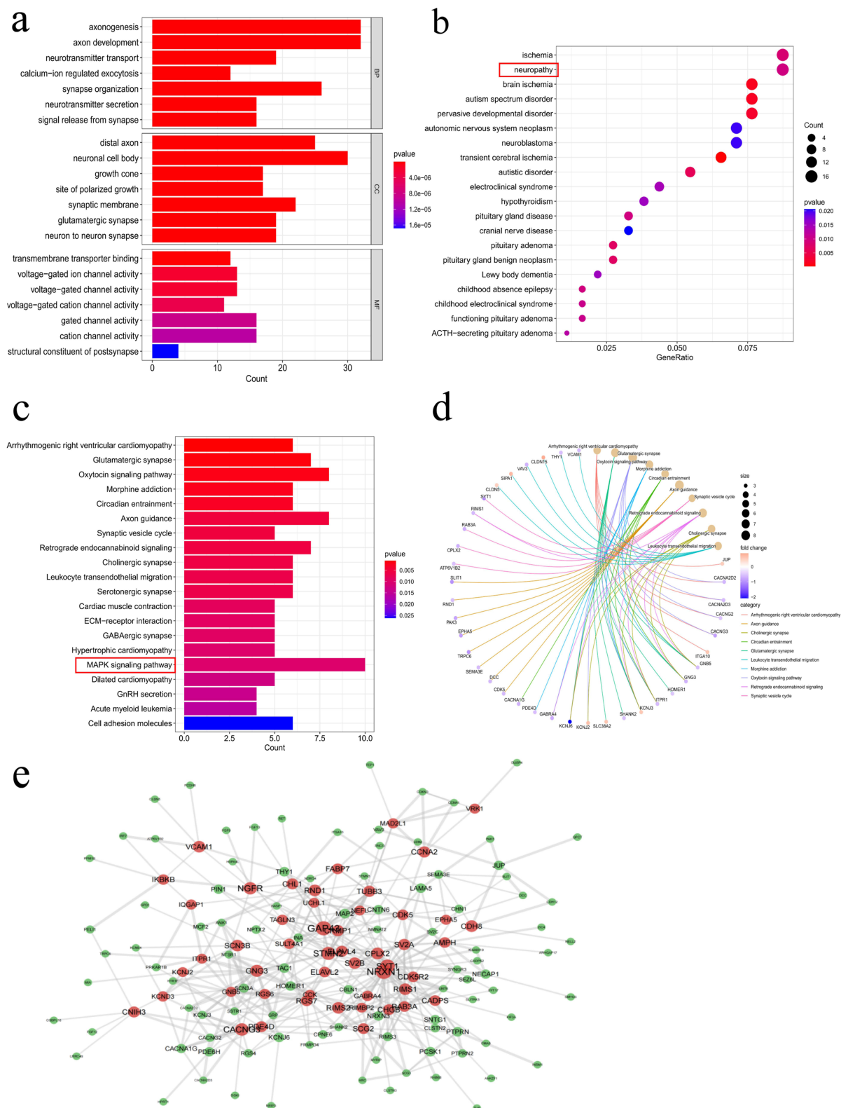
Figure 3 Functional enrichment analysis. (a) Venn diagram showing intersection of DEGs and WGCNA-derived candidate feature genes. (b) Gene Ontology (GO) enrichment analysis of DEGs categorized into biological process (BP), cellular component (CC), and molecular function (MF). (c) Disease Ontology (DO) analysis revealing diseases associated with candidate genes. (d and e) KEGG pathway enrichment analysis highlighting pathways involving candidate feature genes. (f) Protein-protein interaction (PPI) network analysis of candidate feature genes in PD, indicating significant protein interactions.
