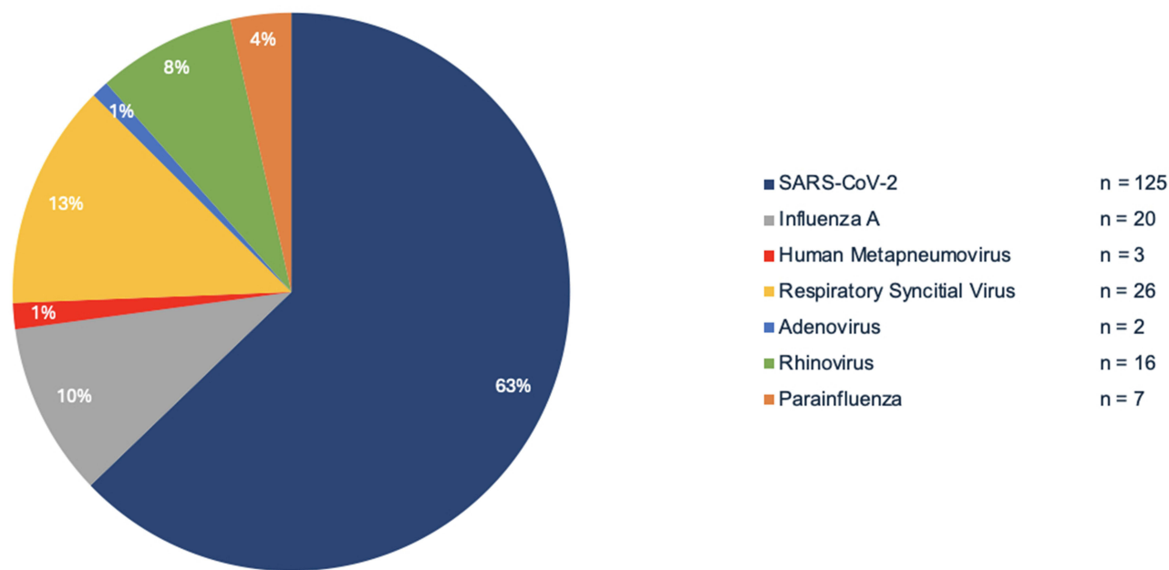
Figure 2 Pie chart demonstrating percentage of cases per respective viral AECOPD.
