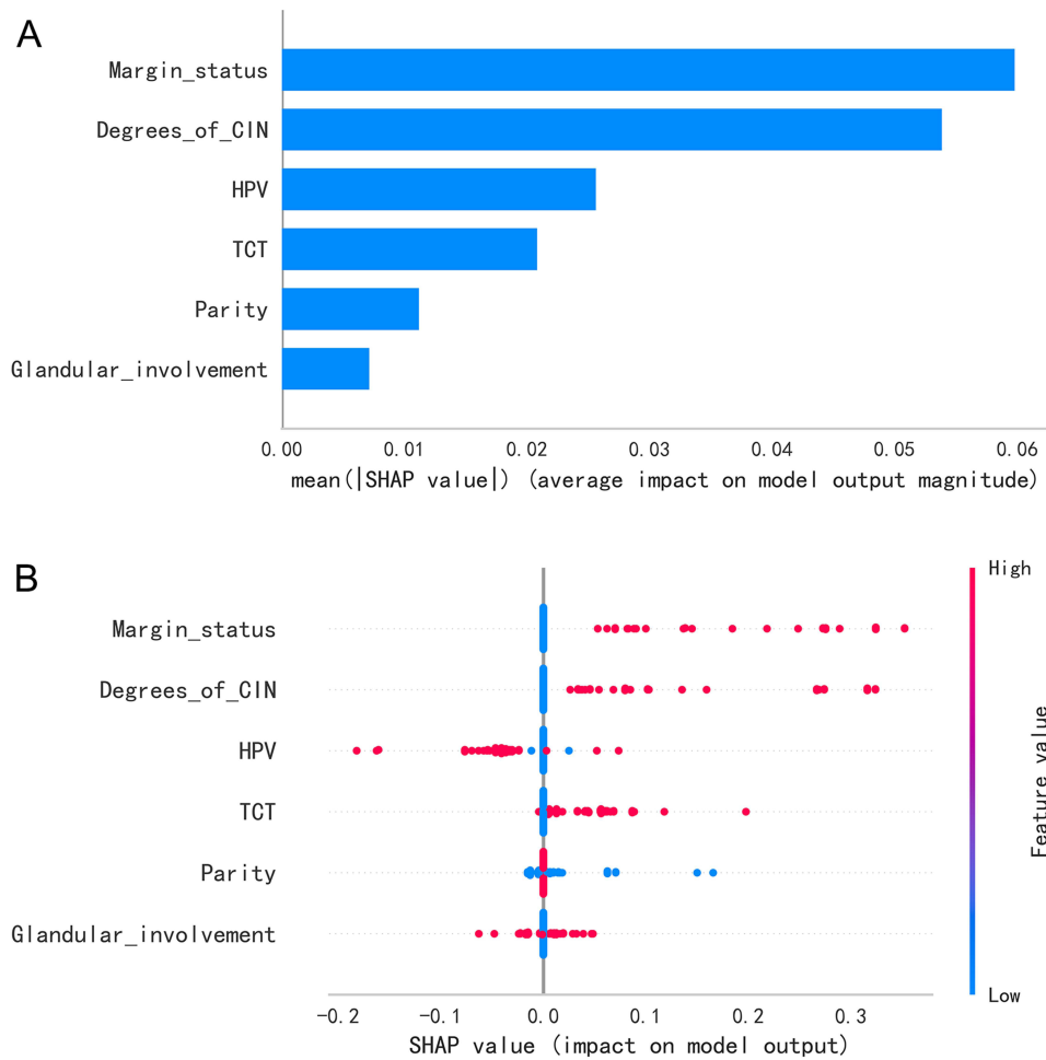
Figure 4 SHAP value analysis of predictive factors in the random forest survival analysis of high-grade cervical intraepithelial neoplasia (CIN) after conization. (A) A graph of the mean SHAP values showing the average impact of each predictor on the model output. (B) A bee swarm plot displaying the individual SHAP values for each predictor across all data points, with color coding according to the feature value.
