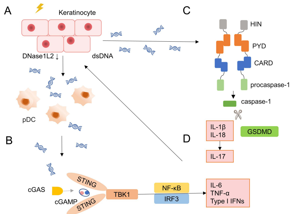
Figure 1 AIM2 and cGAS in psoriasis inflammation. (A). Some factors such as bacteria and virus not only produce pathogen-derived dsDNA but also trigger keratinocytes to release self-dsDNA, which subsequently activate DCs. The downregulated DNase1L2 results in a deficiency in DNA degradation. (B). Activated by dsDNA from keratinocytes and pDCs, cGAS enhances cGAMP production and STING activation. STING oligomerizes and recruits TBK1, which phosphorylates STING and IRF3 to induce type-I IFNs. In addition, STING–TBK1 association also activates NF- \kappa B which induces upregulation of IL-6 and TNF- \alpha . Both type-I IFNs and TNF- \alpha contribute to psoriasis development. (C). AIM2 consists of one or two HIN domains at the C-terminus to detect and bind to cytoplasmic dsDNA, and one PYD at the N-terminus to bind to the PYD of ASC. The CARD of ASC binds to procaspase-1 and fulfills the AIM2 inflammasome complex assembly. Caspase-1 cleaves GSDMD and proIL-1 \beta , proIL-18. IL-1 \beta and IL-18 can upregulate IL-17 expression to promote the progression of psoriasis. (D). Proinflammatory cytokines such as TNF- \alpha and IL-17 facilitate further release of dsDNA from keratinocytes.
