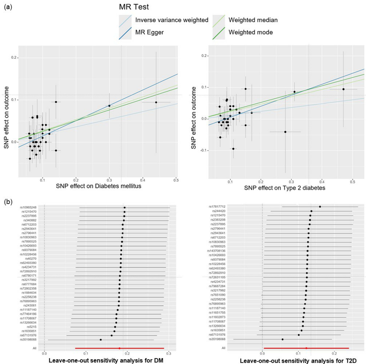
Figure 3 (a) scatter plots for the causality between DM/T2D and vitiligo. (b) leave-one-out plots for the causality between DM/T2D and vitiligo.
