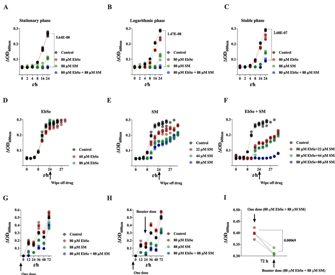
Figure 2 Antibacterial effect of EbSe + SM on M. marinum . M. marinum ATCC BAA-535 cells were cultured until an A_{600}=0.4 , diluted 1:1000 times, and treated with EbSe + SM. (A–C). Cell viability was represented by measuring A_{600} . The growth curves showed a synergistic antibacterial effect of EbSe + SM on M. marinum . Cell viability was represented by measuring A_{600} . (A) Stationary phase ( A_{600}=0.2 ). (B) Logarithmic growth phase ( A_{600}=0.6 ). (C) Stable phase ( A_{600}=1.0 ). (D–F) The PAE effect of EbSe + SM against M. marinum . (D) EbSe. (E) SM. (F) EbSe + SM. (G–I) The bacteriostasis effect of EbSe + SM against M. marinum . (G) One-dose administration. (H) Two-dose administration. (I) One-dose VS two-doses. Cell viability was represented by measuring A_{600} . N = 5 independent observations per group, and triplicate biological replications were applied. Data are presented by Student's t test, p<0.05 constitutes statistical significance.
