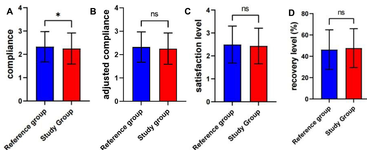
Figure 1 Subjective feedback from the patients. (A and B) Patients' compliance in the reference group ( n = 483 ) was higher than the study group ( n = 549 ), but the difference gone with adjusted cases in the study group ( n=521 ). (C and D) The satisfaction level and the recovery level were similar between the two groups.
