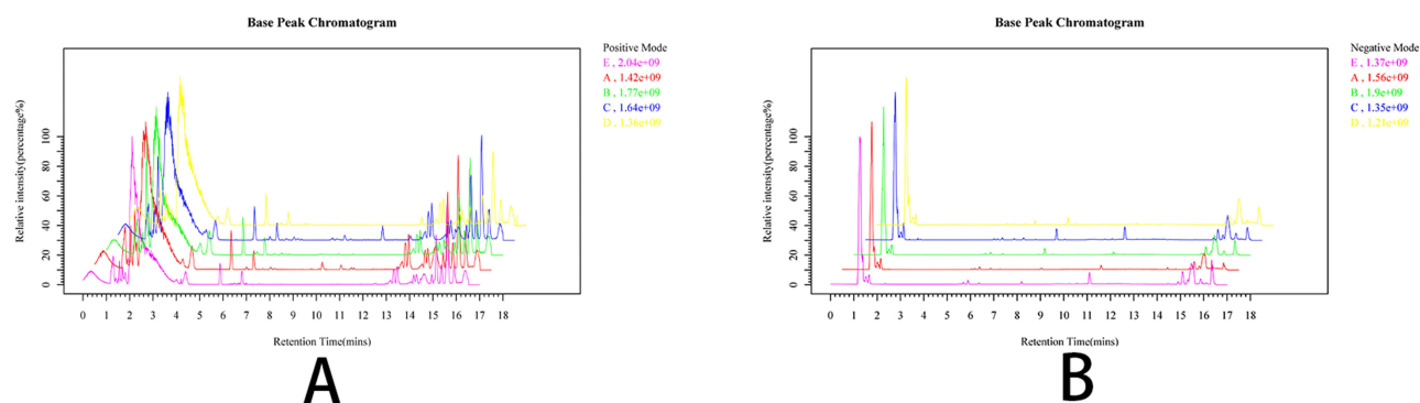
Figure 1 Base peak chromatogram of CKD patients and control group obtained with LC-MS positive (A), negative (B) ionization mode.
