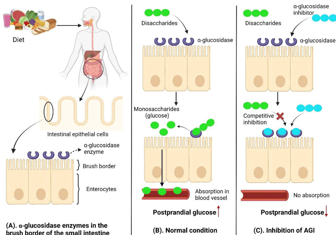
Figure 2 Mechanism of \alpha -glucosidase inhibition. (A). \alpha -glucosidase enzymes in the brush border of the small intestine; (B). normal condition of \alpha -glucosidase enzymes without inhibition of AGI; (C). condition of \alpha -glucosidase enzyme inhibited by AGI. Created with BioRender.com. 84,85
