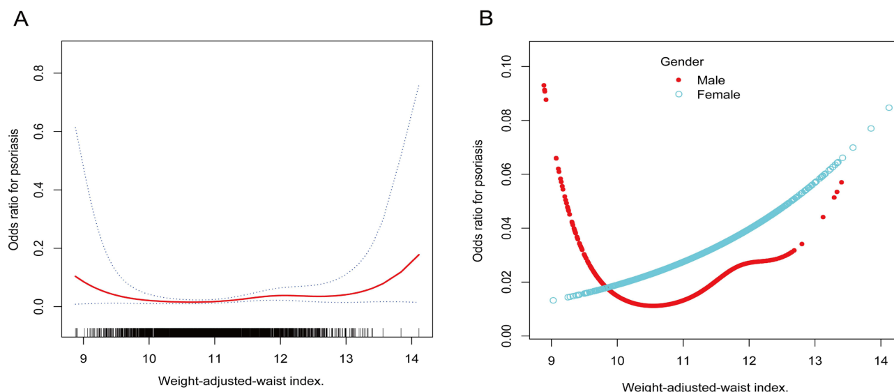
Figure 2 (A) Detected Smooth Curve Fitting With the use of the generalized additive model, a nonlinear positive connection between WWI and psoriasis was found. (B) The association between WWI and psoriasis stratified by gender.
