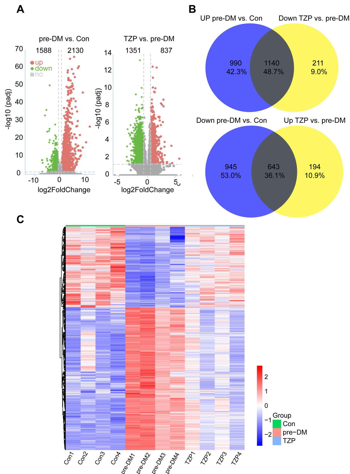
Figure 6 DEGs regulated by TZP. (A) Volcano plots of differentially expressed genes (DEGs) in pre-DM/Con and TZP/pre-DM. (B) 1140 down-regulated and 643 up-regulated DEGs by treatment with TZP. (C) Heatmap of 1783 crossed-differently expressed genes in the three groups.
