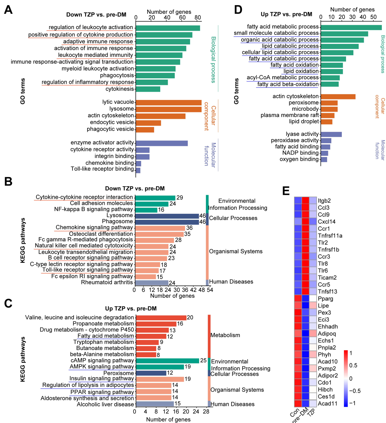
Figure 7 Enrichment results of DEGs. (A and B) GO and KEGG annotations of common DEGs from the comparison of TZP downregulation vs pre-DM (red, down-regulated). (C and D) KEGG and GO annotations of common DEGs from the comparison of TZP upregulation vs pre-DM (blue, up-regulated). (E) Heatmap of prediabetes-related DEGs for the three experimental groups.
