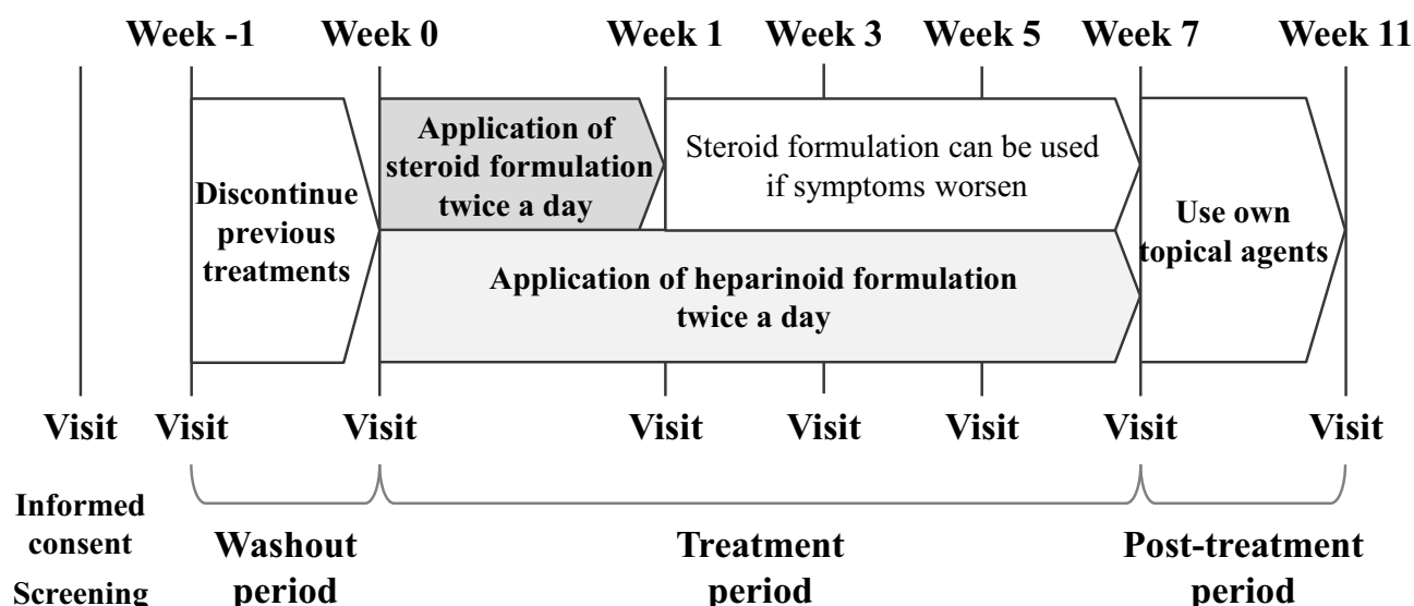
Figure 1 Study design.
