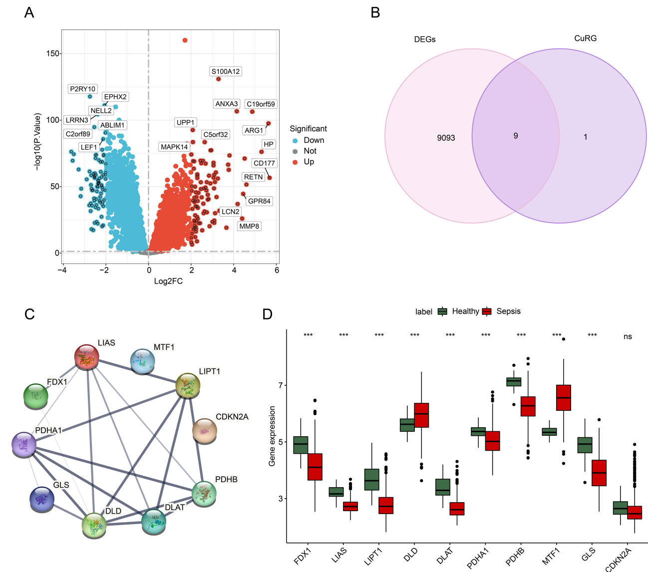
Figure 1 Difference analysis of CuRGs between healthy and sepsis groups. (A) Difference analysis of healthy and sepsis groups in GSE65682. The cutoff for selecting DEGs is set at P < 0.05 . (B) Identification of DE-CuRGs. (C) PPI network displays the relationship between 10 CuRGs. (D) Expression profile of 10 CuRGs in the healthy and sepsis groups. *** P < 0.001 ; ns: P > 0.05 .
