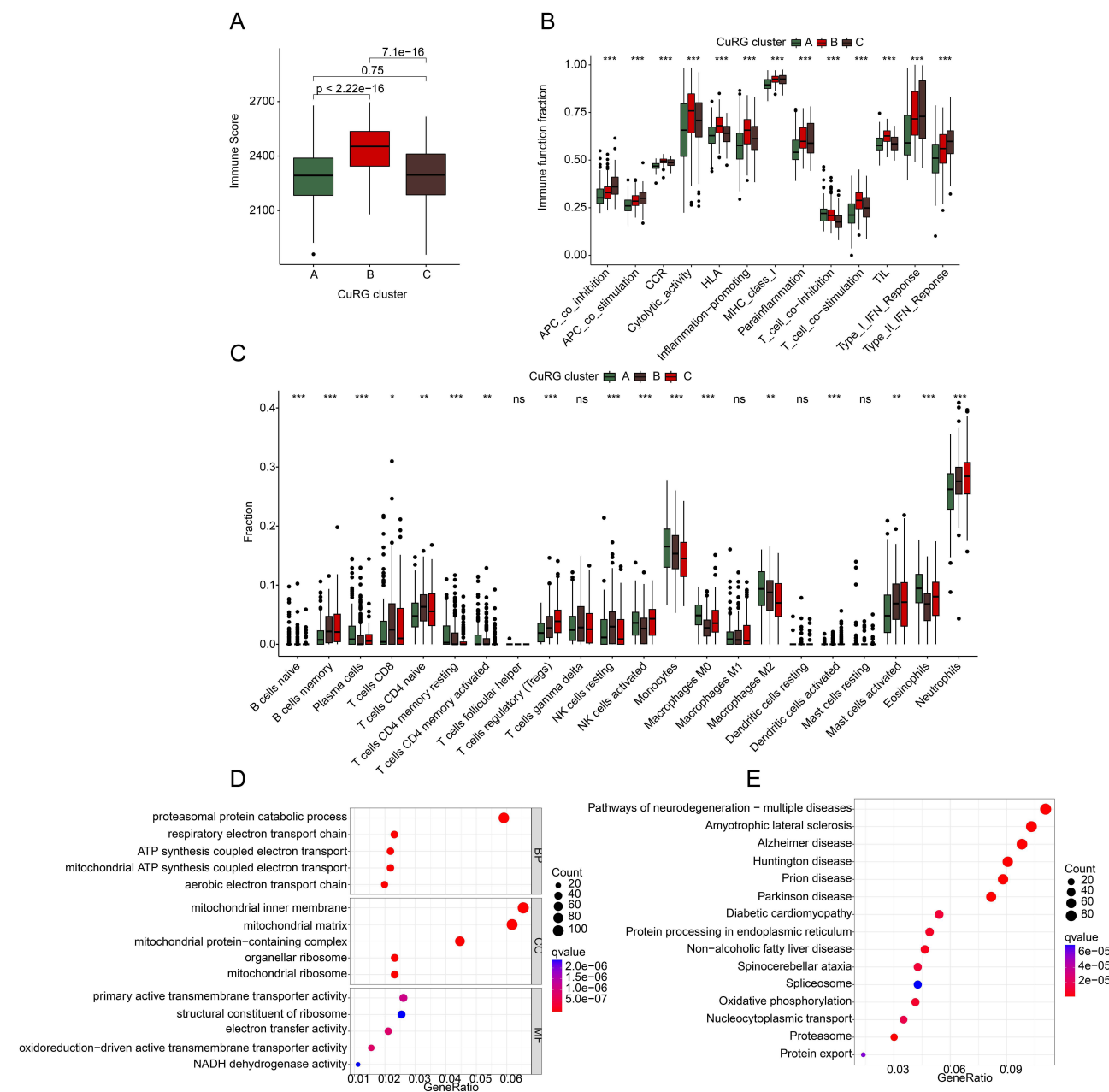
Figure 6 Immune analysis and differential enrichment analysis of CuRGs molecular subtypes in sepsis. (A) Immune scores of CuRGs molecular subtypes in sepsis. (B) Functional analysis of immune functions in CuRGs molecular subtypes in sepsis. (C) Infiltration analysis of immune cells in CuRGs molecular subtypes in sepsis. Differential genes of CuRGs molecular subtypes in sepsis were subjected to (D) GO analysis and (E) KEGG enrichment analysis. * P < 0.05 ; ** P < 0.01 ; *** P < 0.001 ; ns: P > 0.05 .
