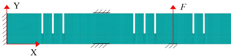
Figure 38 Schematic diagram of force calculation when PIP is individually driven.
