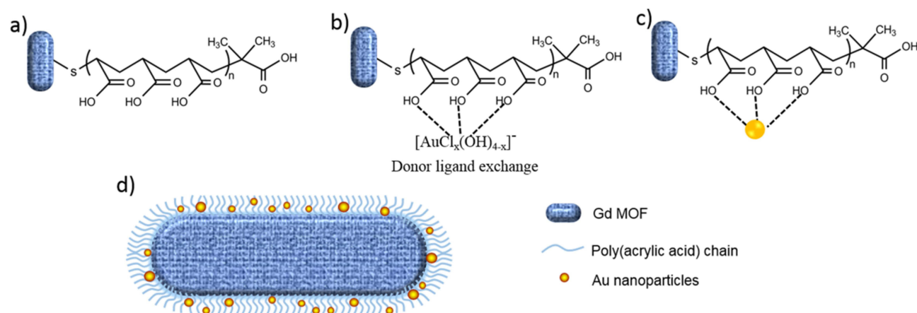
Figure 3 The synthetic strategy for fabricating hybrid GdMOF-PAA-Au nanostructures involves a sequential multi-step process: (a) the initial deposition of poly(acrylic acid) (PAA) onto the surface of gadolinium metal-organic framework (GdMOF) nanostructures, (b) the subsequent adsorption of gold (Au) ions onto the PAA-functionalized GdMOF nanostructures, and (c) the reduction of the Au ions, culminating in the formation of gold nanoparticles (AuNPs) firmly entrapped within the PAA matrix on the nanostructure's surface. (d) A schematic delineation of the hybrid nanostructure is presented, where the GdMOF core is depicted in blue, the entangled PAA chains in blue, and the incorporated AuNPs are illustrated in gold, demonstrating the complex's structural composition and the spatial distribution of its constituents. Reprinted with permission from Tian C, Zhu L, Lin F, Boyes SG. Poly(acrylic acid) Bridged gadolinium metal-organic framework-gold nanoparticle composites as contrast agents for computed tomography and magnetic resonance bimodal imaging. ACS Appl Mater Inter. 2015;7(32):17765–17775. Copyright 2015 American Chemical Society. 11
