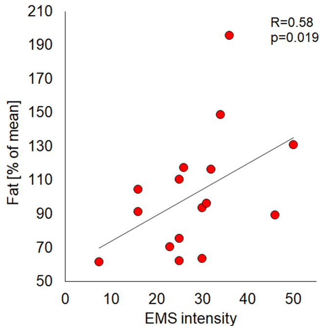
Figure 9 Correlation between the maximum intensity of the applied EMS stimulus and body fat mass expressed as a percentage of the average fat mass for women of a certain height.
