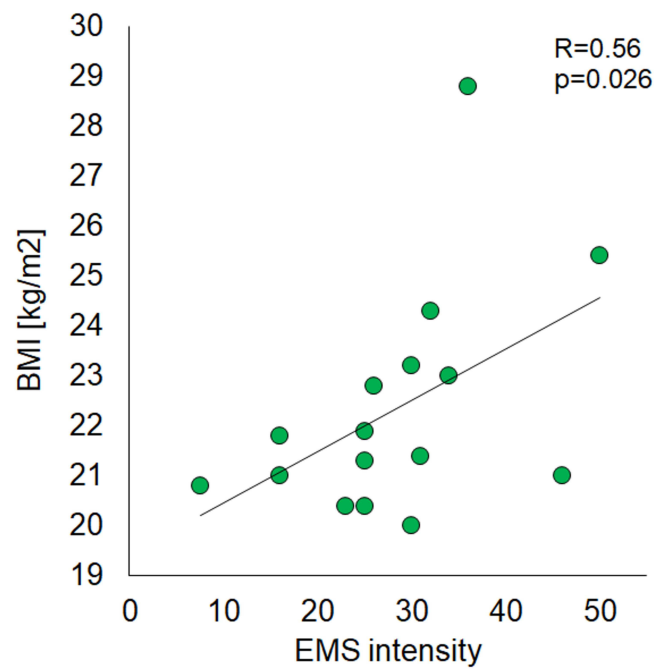
Figure 5 Correlations between the maximum EMS intensity and BMI.
