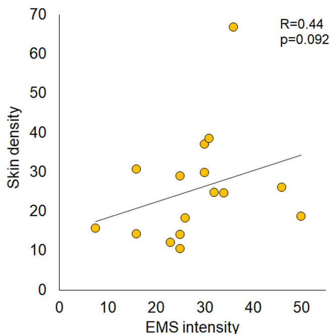
Figure 13 Correlation between the maximum intensity of the applied EMS stimulus and skin density.
