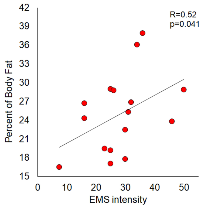
Figure 10 Correlation between the maximum intensity of the applied EMS stimulus and percentage of body fat in relation to the weight.
