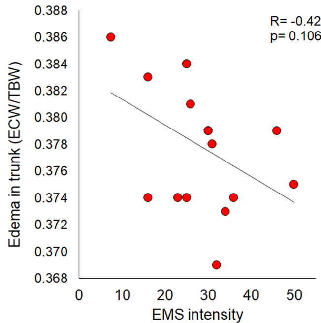
Figure 12 Correlation between the maximum intensity of the applied EMS stimulus and trunk edema index.
