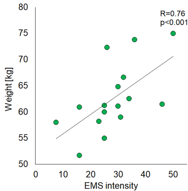
Figure 3 Correlations between the maximum EMS intensity and body weight.
