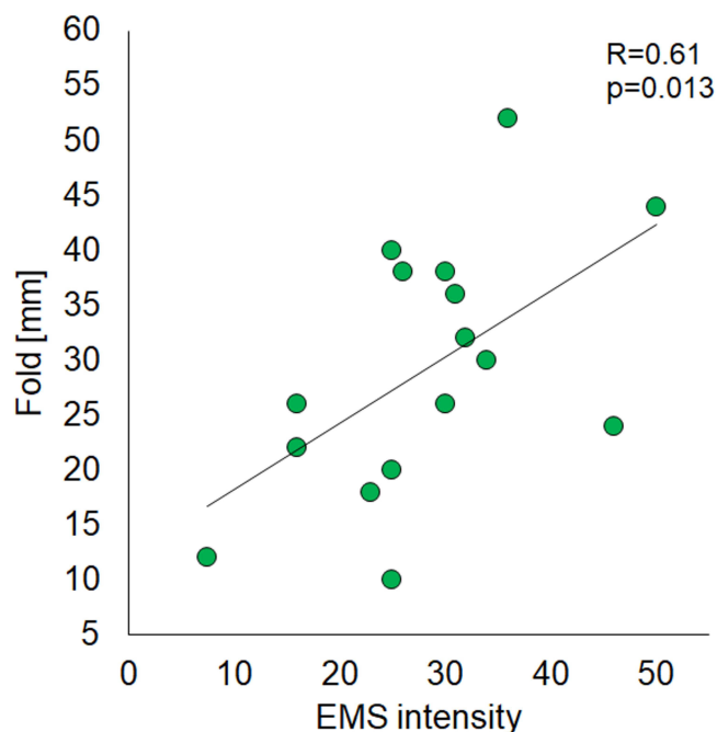
Figure 7 Correlations between the maximum EMS intensity and skinfold thickness.
