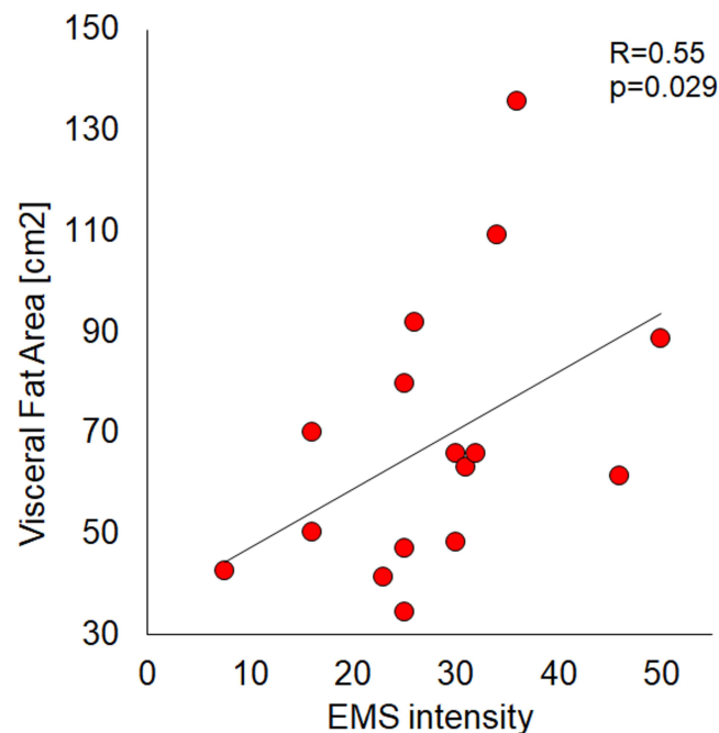
Figure 11 Correlation between the maximum intensity of the applied EMS stimulus and visceral fat area.
