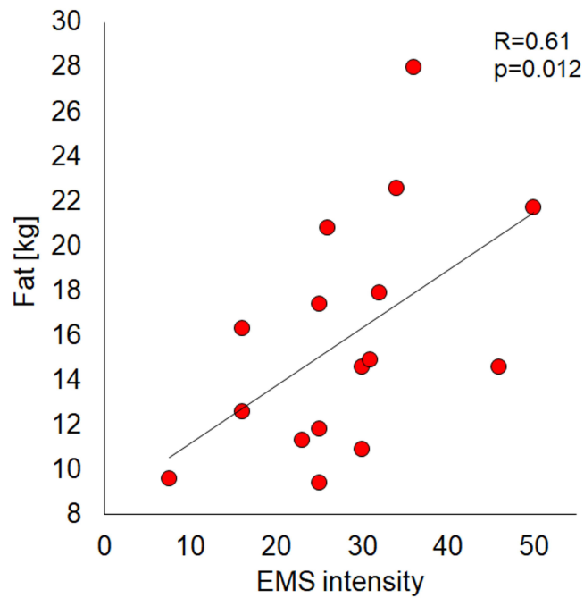
Figure 8 Correlation between the maximum intensity of the applied EMS stimulus and body fat mass.
