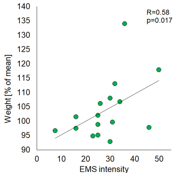
Figure 4 Correlations between the maximum EMS intensity and body weight compared to the population mean for certain height.
