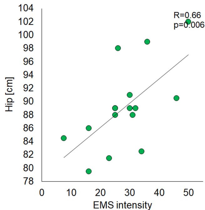
Figure 6 Correlations between the maximum EMS intensity and Hip circumference.
