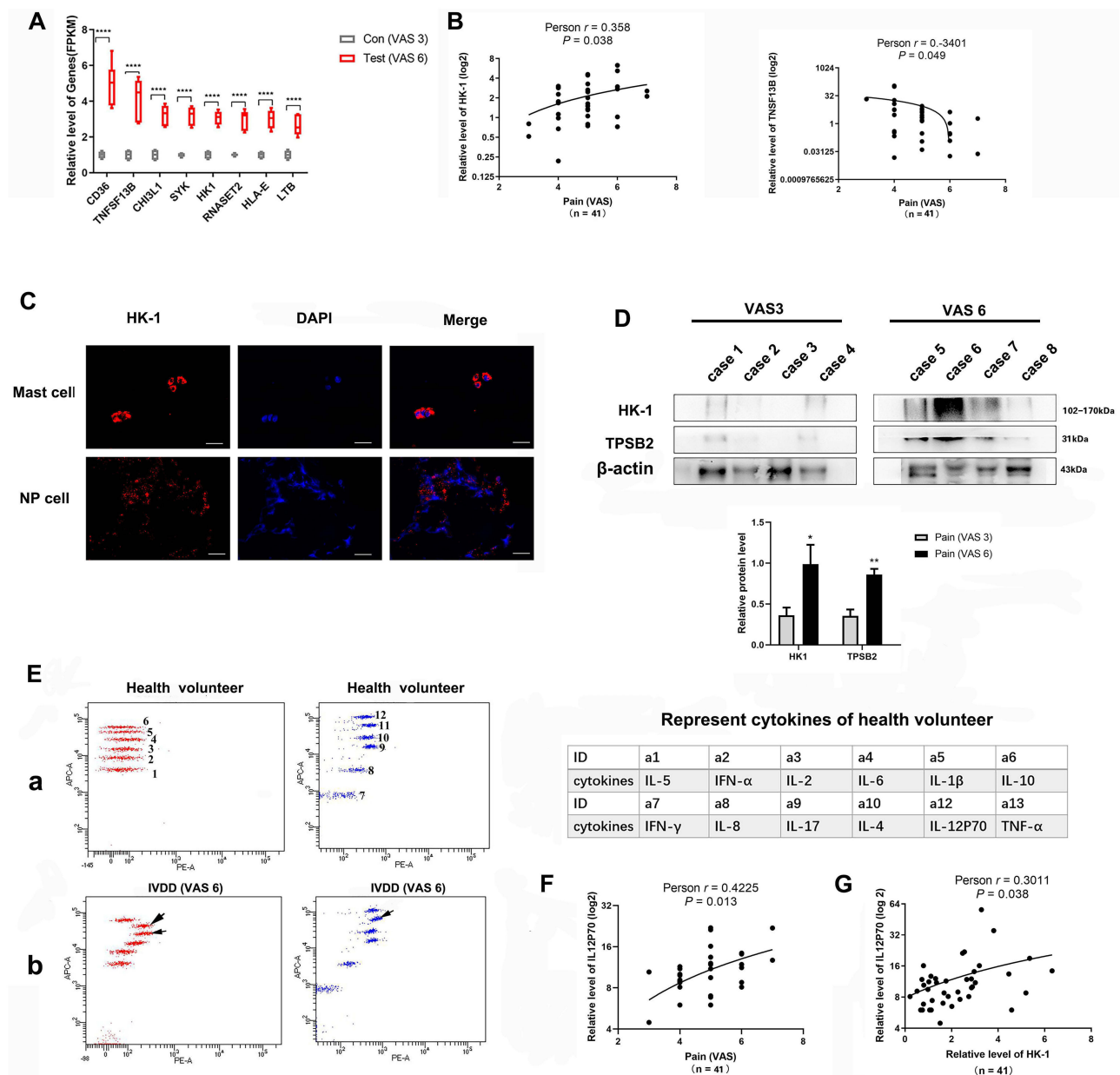
Figure 5 The high expression of the mast cell-related gene HK-I is closely correlated with discogenic LBP. (A) The expression of mast cell-related genes from RNA-seq results in VAS3 and VAS6 NP tissues. **** P < 0.0001 . (B) The relationship between HK-I and TNSF13B with discogenic LBP in 41 NP tissues from IVDD patients of various grades. (C) The localization of HK-I in mast and NP cells. (D) The protein levels (up) and histogram of gray value statistics (down) of HK-I, mast cell TPSB2 in VAS3 and VAS6 NP tissues * P < 0.05 , ** P < 0.01 . (E) Levels of 12 cytokines in the peripheral venous blood of 41 IVDD patients. a. 12 cytokines distribution in flow cytometry of healthy volunteers act as stand curve (left). The names corresponding to the distribution locations of the 12 cytokines (right table). b. 12 cytokines distribution in flow cytometry of VAS6 - IVDD patient. (F) A high expression level of IL-12P70 is closely related to LBP. (G) Tissue HK-I expression is correlated with blood IL-12P70 expression.
