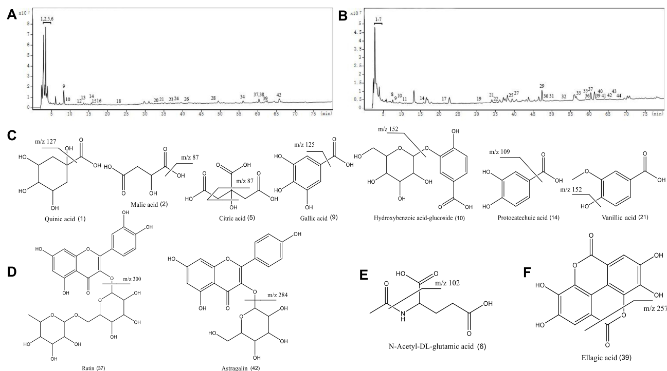
Figure 3 Ion chromatogram of AEMC (A) and AELLF (B) analyzed by HPLC-Q-TOF-MS/MS, and the structural formula of the 11 common components (C–F). (A) The total ion chromatogram of AEMC. (B) The total ion chromatogram of AELLF. (C) The structural formulas of seven organic acids. (D) The structural formulas of two flavonoids. (E) The structural formulas of amino acid. (F) The structural formulas of tannin. 9, gallic acid; 17, neochlorogenic acid; 19, chlorogenic acid; 22, cryptochlorogenic acid; 23, caffeic acid; 35, hyperoside; 37, rutin; 38, rosmarinic acid; 42, astragalin.
