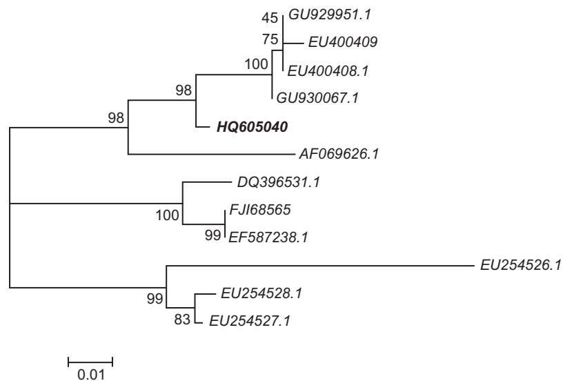
Figure 4 Phylogeny of Hepaticystis species using mitochondrial cytochrome b genes. Numbers on branches are percentages of 1000 bootstrap supporting a given branch. Sequences from Hepaticystis species are listed along with their respective GenBank accession numbers. HQ605040 was newly obtained in this study.
