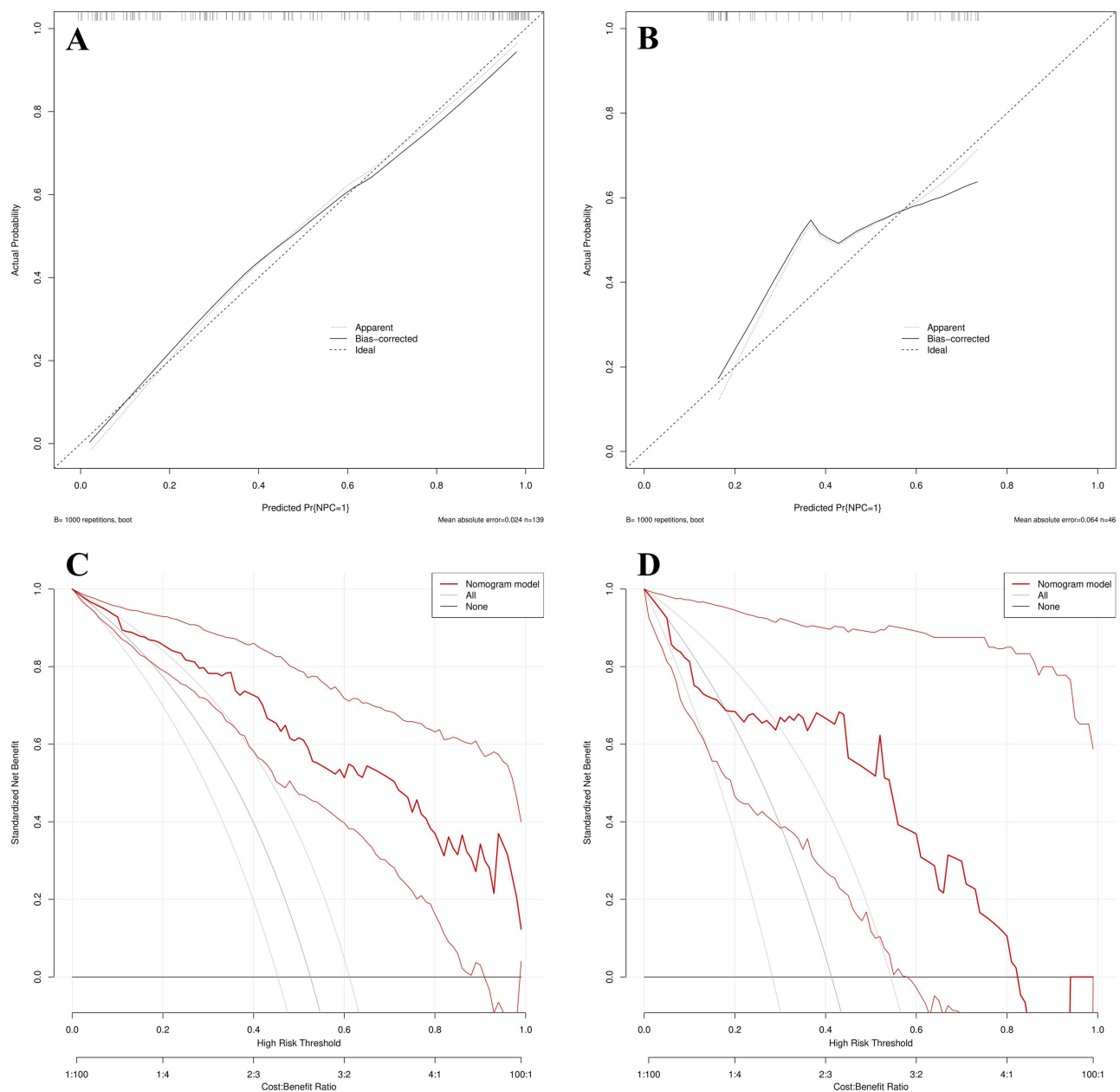
Figure 3 Calibration and DCA curve of the nomogram. (A) Calibration curve of the training cohort; (B) Calibration curve of the validation cohort, the dashed line represents the original performance, and the solid dashed line represents the performance during validation by bootstrapping ( B = 1000 repetitions). (C) DCA curve of the training cohort; (D) DCA curve of the validation cohort. None: All patients receive no specific intervention, representing the scenario where the Nomogram model is not applied for prediction, indicating that all patients are not diagnosed with NPC. ALL: The predictive results of the Nomogram model are used to intervene in all patients, representing the scenario where all patients are diagnosed with NPC. The red line illustrates the net benefit of the Nomogram model relative to the default strategy at different threshold probabilities.
