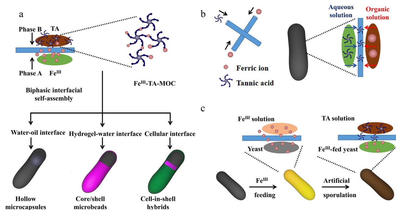
Figure 4 (a) Schematic representation of interfacial supramolecular self-assembly of Fe III and TA at various interfaces. Fe III ions are preloaded into one phase (Phase A), and the supramolecular self-assembly is induced at the interface of two immiscible phases by TA in the other phase (Phase B). (b) Schematic representation for formation of Fe III -TA-MOC hollow nanoshell. (c) Schematic representation for self-responsive Fe III -TA-MOC nanoshell formation on baker's yeast.
