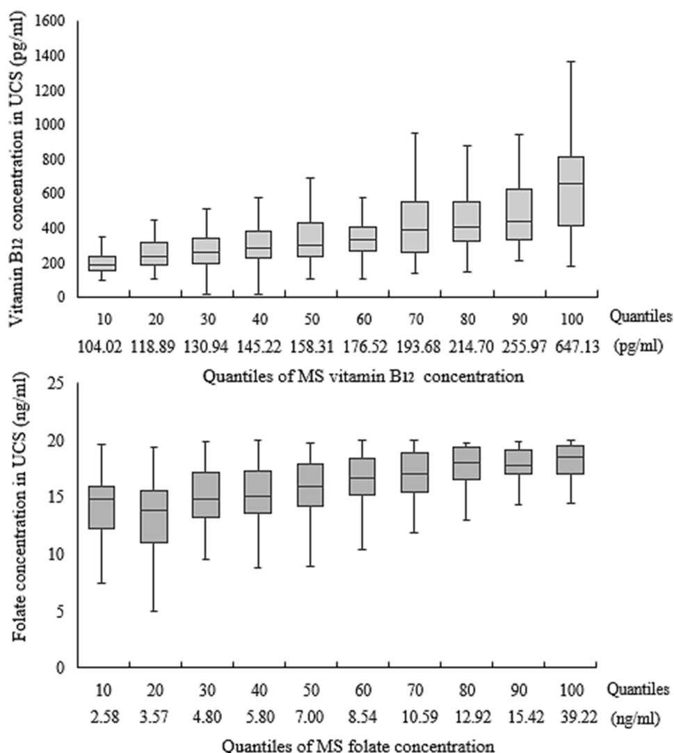
Figure 1 The UCS concentrations at quantiles of MS vitamin B 12 and folate.
