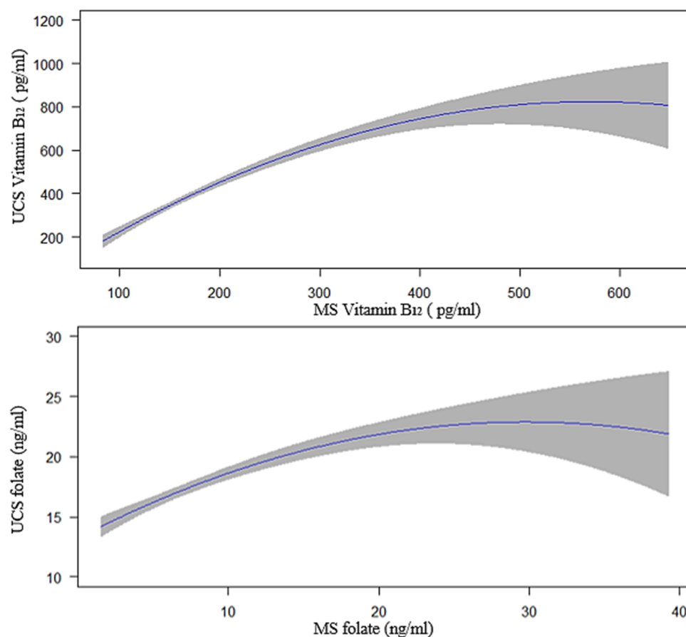
Figure 2 The curve relation between MS and UCS concentration of folate and vitamin B 12 .
