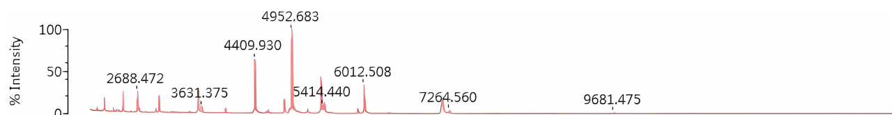
Figure 4 Mass spectrogram of Weissella confusa .
