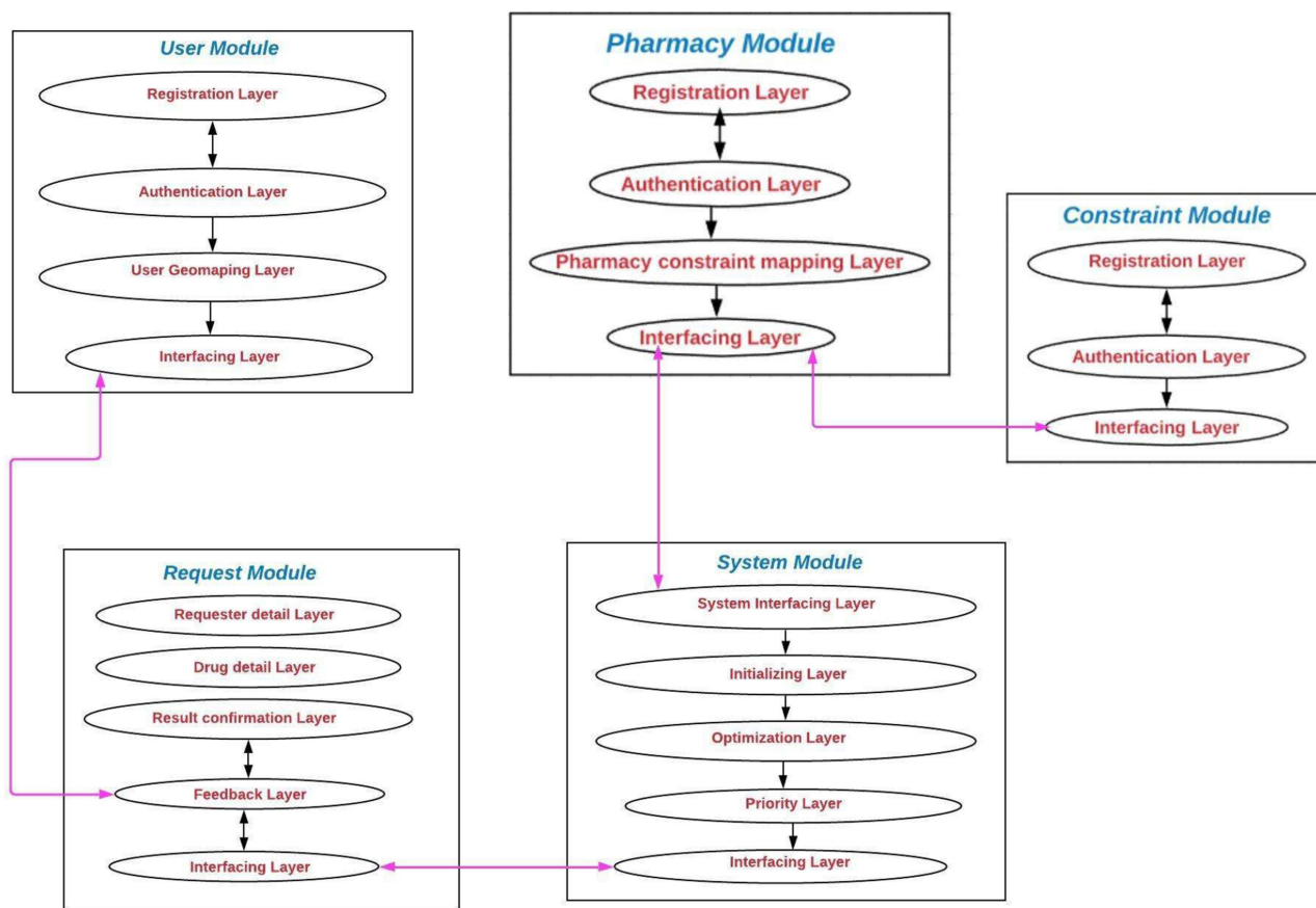
Figure 2 Architecture of the constraint optimization framework.
