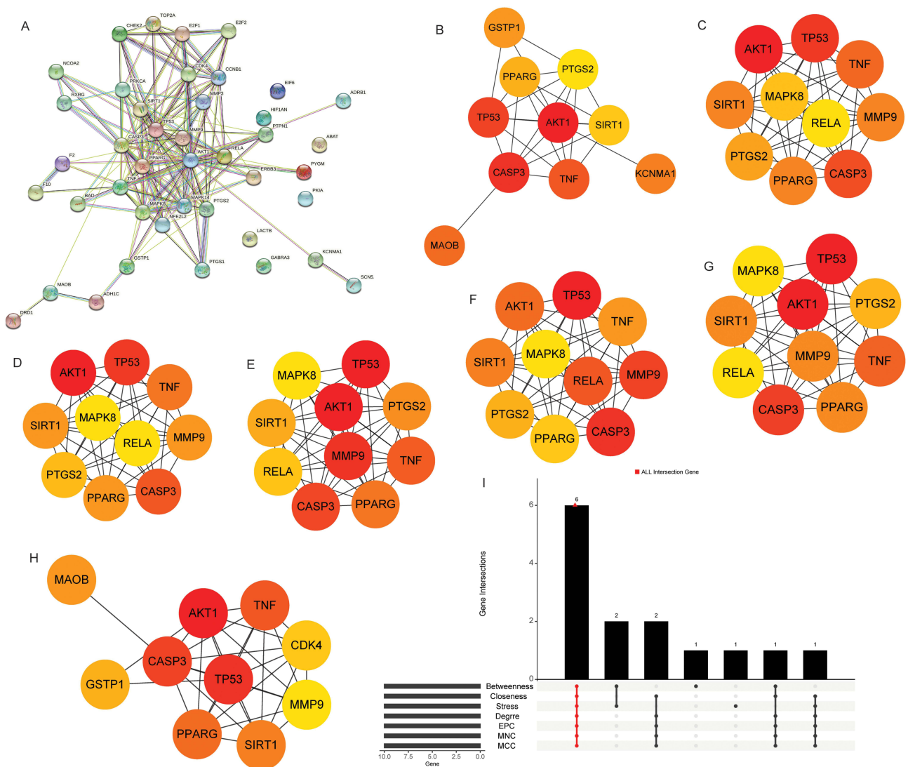
Figure 4 Identification of hub differentially expressed target genes. (A) PPI network of 42 differentially expressed target genes; (B) PPI network of top 10 node genes in Betweenness algorithm. The darker the color, the more important the gene. (C) PPI network of top 10 node genes in Closeness algorithm. The darker the color, the more important the gene. (D) PPI network of top 10 node genes in Degree algorithm. The darker the color, the more important the gene. (E) PPI network of top 10 node genes in Edge Percolated Component (EPC) algorithm. The darker the color, the more important the gene. (F) PPI network of top 10 node genes in Maximal Clique Centrality (MCC) algorithm. The darker the color, the more important the gene. (G) PPI network of top 10 node genes in Maximum Neighborhood Component (MNC) algorithm. The darker the color, the more important the gene. (H) PPI network of top 10 node genes in Stress algorithm. The darker the color, the more important the gene. (I) Screening of hub differentially expressed target genes.
