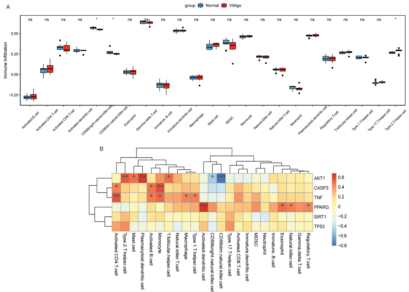
Figure 6 Immune cell infiltration in the IME of non-segmental vitiligo. (A) Infiltration of 23 immune cells in the IME of non-segmental vitiligo; (B) Correlation analysis between immune cells and hub differentially expressed target genes. ns represent no significant difference; *Represent P<0.05; **Represent P<0.01; ***Represent P<0.001; ns represent no statistical significance.
