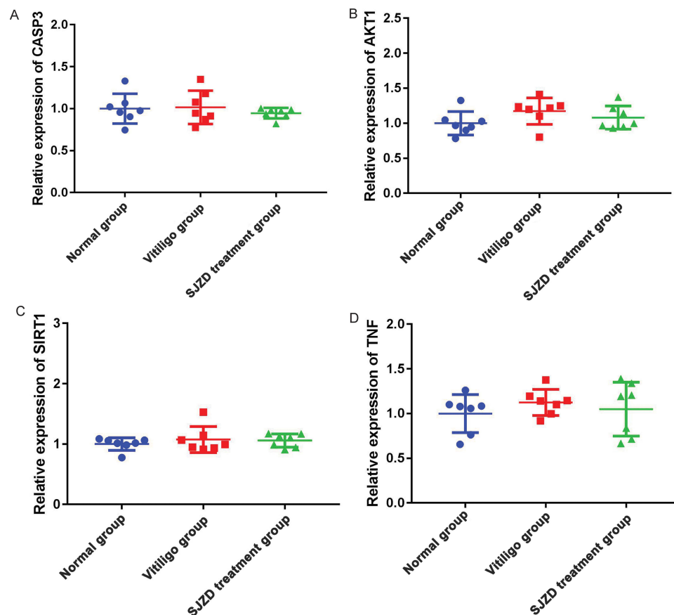
Figure 8 Real-time PCR detection of CASP3 (A), AKT1 (B), SIRT1 (C) and TNF (D).
