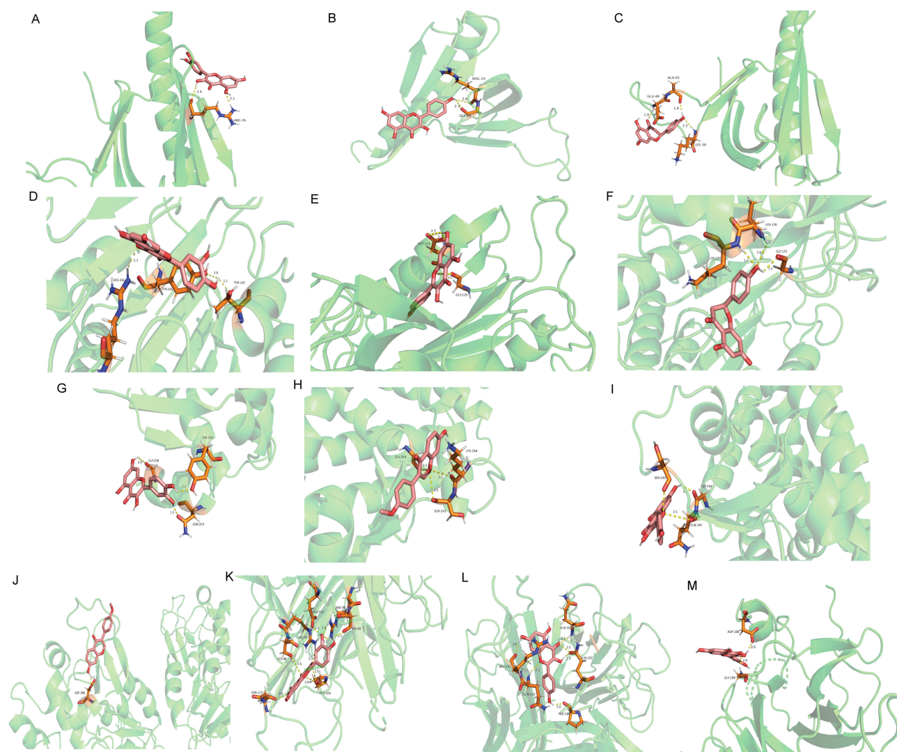
Figure 7 Molecular docking diagram of the active compounds with the hub differentially expressed target genes. (A) Molecular docking diagram of AKT1 and quercetin; (B) Molecular docking diagram of AKT1 and kaempferol; (C) Molecular docking diagram of AKT1 and naringenin; (D) Molecular docking diagram of CASP3 and quercetin; (E) Molecular docking diagram of CASP3 and kaempferol; (F) Molecular docking diagram of CASP3 and naringenin; (G) Molecular docking diagram of PPARG and quercetin; (H) Molecular docking diagram of PPARG and formononetin; (I) Molecular docking diagram of PPARG and kaempferol; (J) Molecular docking diagram of SIRT1 and formononetin; (K) Molecular docking diagram of TNF and quercetin; (L) Molecular docking diagram of TNF and kaempferol; (M) Molecular docking diagram of TP53 and quercetin.
