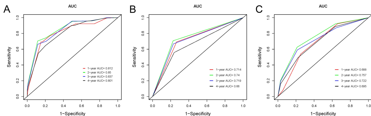
Figure 4 The predictive effectiveness of the novel nomogram, IPI system and NCCN-IPI system. (A) The 1-year, 2-year, 3-year and 4-year AUC of the novel nomogram was 0.812, 0.85, 0.837, and 0.801, respectively. (B) The 1-year, 2-year, 3-year and 4-year AUC of IPI system was 0.714, 0.74, 0.719, and 0.66, respectively. (C) The 1-year, 2-year, 3-year and 4-year AUC of NCCN-IPI system was 0.688, 0.757, 0.722, and 0.695, respectively.
