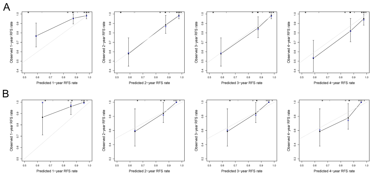
Figure 3 The calibration plots of nomogram in training cohort (A) and validation cohort (B) showed the predicted RFS rate on the x axis and the observed RFS on the y axis. Abbreviation: RFS, recurrence-free survival.
