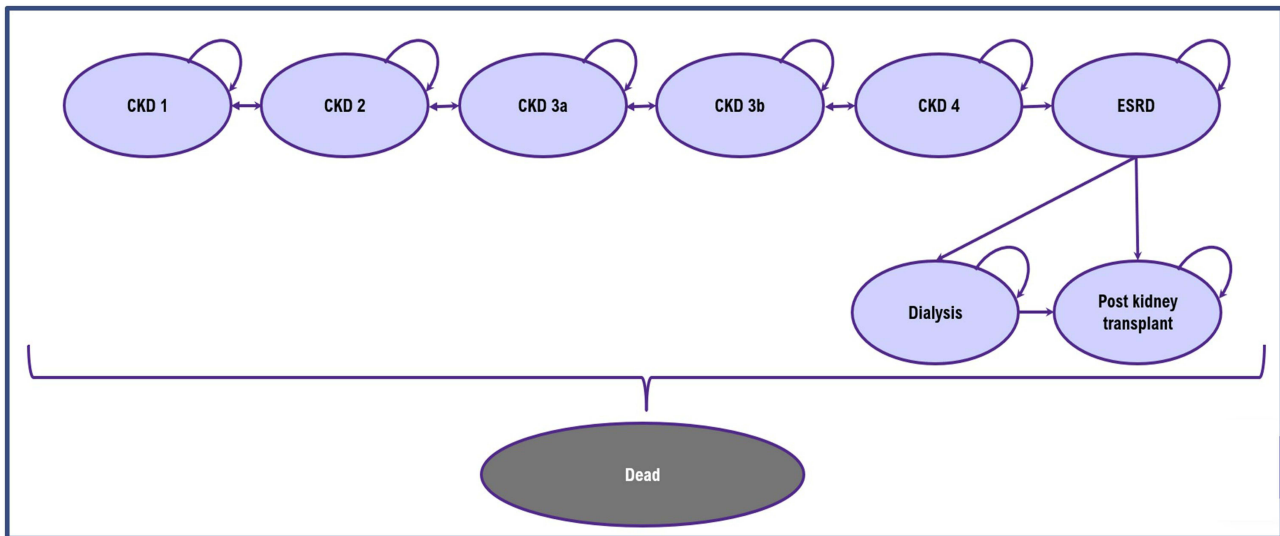
Figure 1 Semi-Markov model structure.
