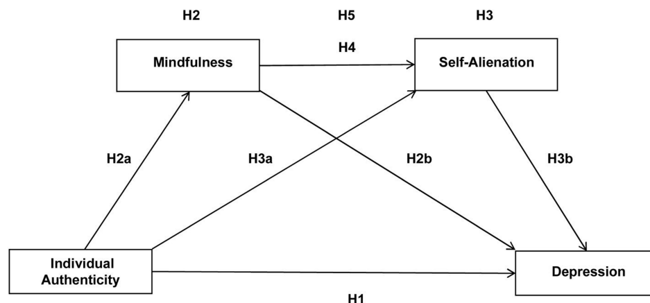
Figure 1 Theoretical hypothesis.
