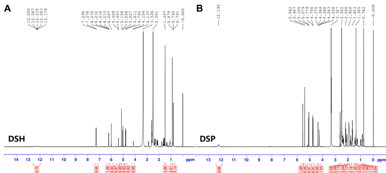
Figure 2 1 H-NMR spectrum of DSH (A) and DSP (B).
