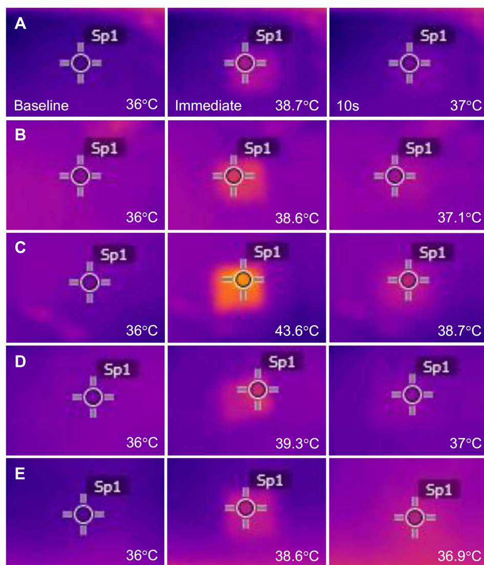
Figure 2 Thermal imaging camera study. Images were captured at baseline, immediately, and 10s after bipolar RF treatment at a frequency of 2 MHz. The experimental settings were (A) a power of 4V, a conduction time/pulse pack of 200 msec, and a single pulse pack; (B) 12V, a conduction time/pulse pack of 200 msec, and a single pulse pack; (C) 12V, a conduction time/pulse pack of 600 msec, and a single pulse pack; (D) 12V, a conduction time/pulse pack of 100 msec, two pulse packs, an off-time between pulse packs of 50 msec, and a total conduction time of 200 msec; and (E) 12V, a conduction time/pulse pack of 100 msec, two pulse packs, an off-time between pulse packs of 20 msec, and a total conduction time of 200 msec. The thermometric values of baseline tissue were adjusted to 36°C.
