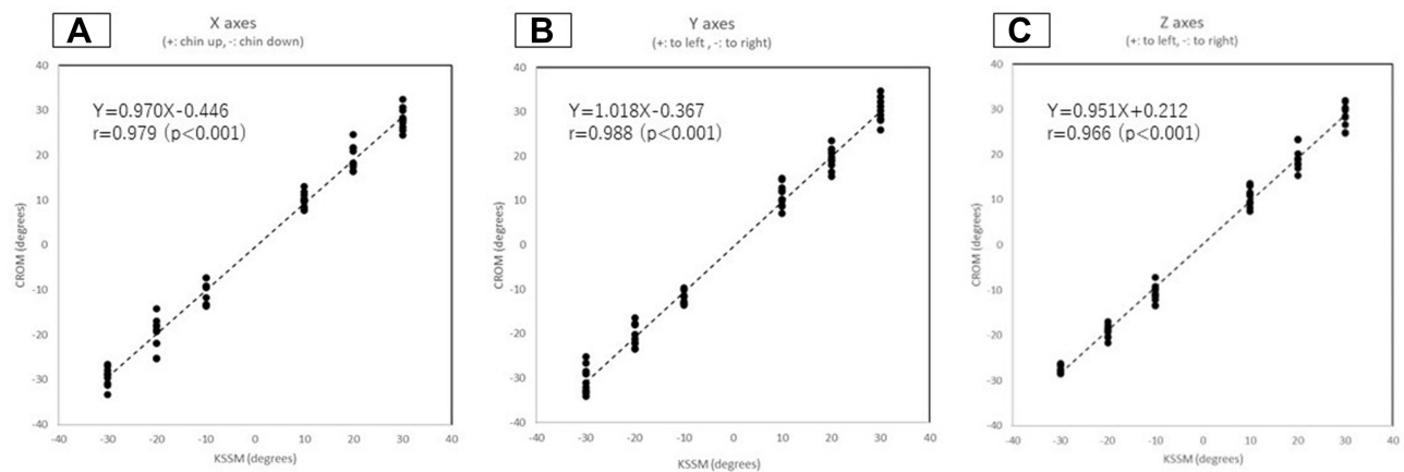
Figure 3 The Spearman correlation coefficients between KSSM and the CROM device for X (3A), Y (3B), and Z axes (3C). A significant correlation was observed for the relationship between the measurements of KSSM and the CROM for all three head movements (chin-up/down: r=0.979 (95% CI: 0.965–0.988), face turn: r=0.988 (95% CI: 0.980–0.993), and head tilt: r=0.966 (95% CI: 0.944–0.980).
