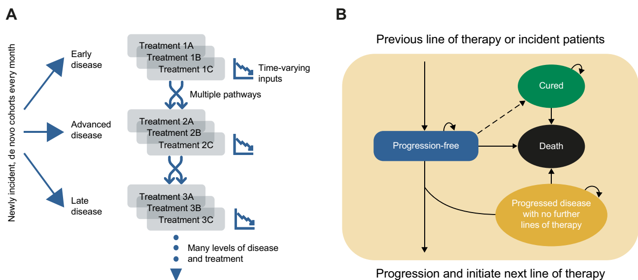
Figure 2 (A) Multi-stage model structure and (B) Markov structure within individual treatments.
