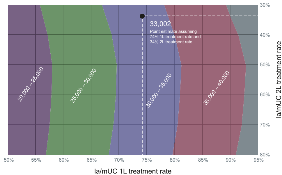
Figure 5 Sensitivity analysis: contour plots of US 2022 la/mUC annual treated prevalence.
