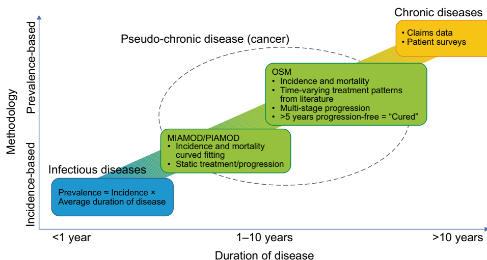
Figure 1 Methods of estimating population size.
