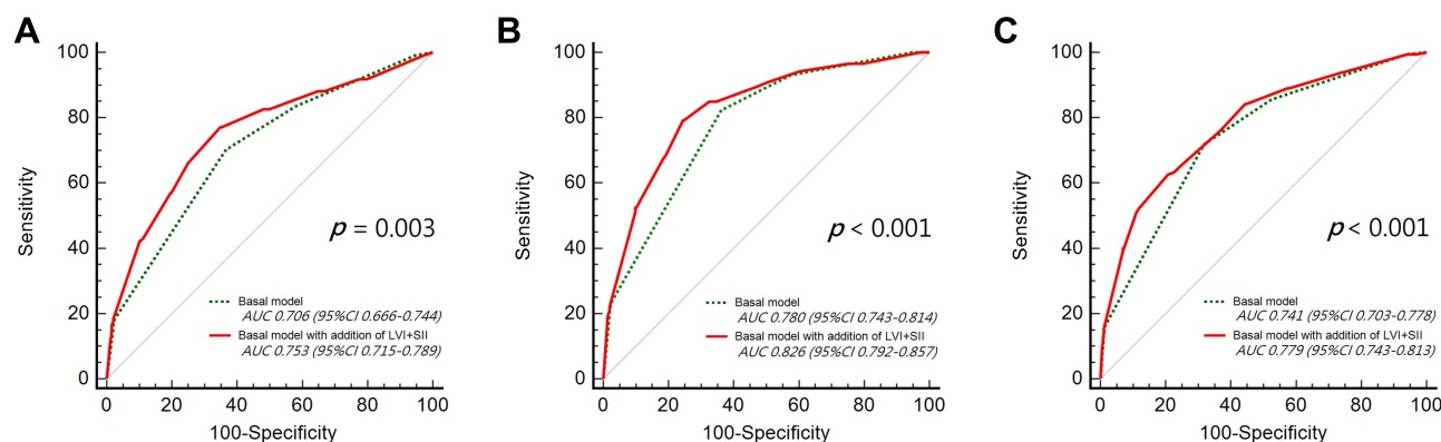
Figure 3 ROC analyses for predictive accuracy of overall survival (A), cancer-specific survival (B), and progression-free survival (C) in UTUC patients according to the basal model (green dot line) and adding LVI and SII to the basal model (red solid line).
