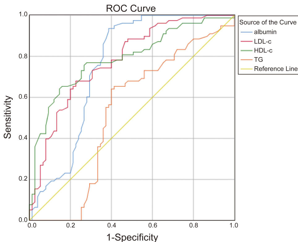
Figure 3 The ROC curves of four markers.
