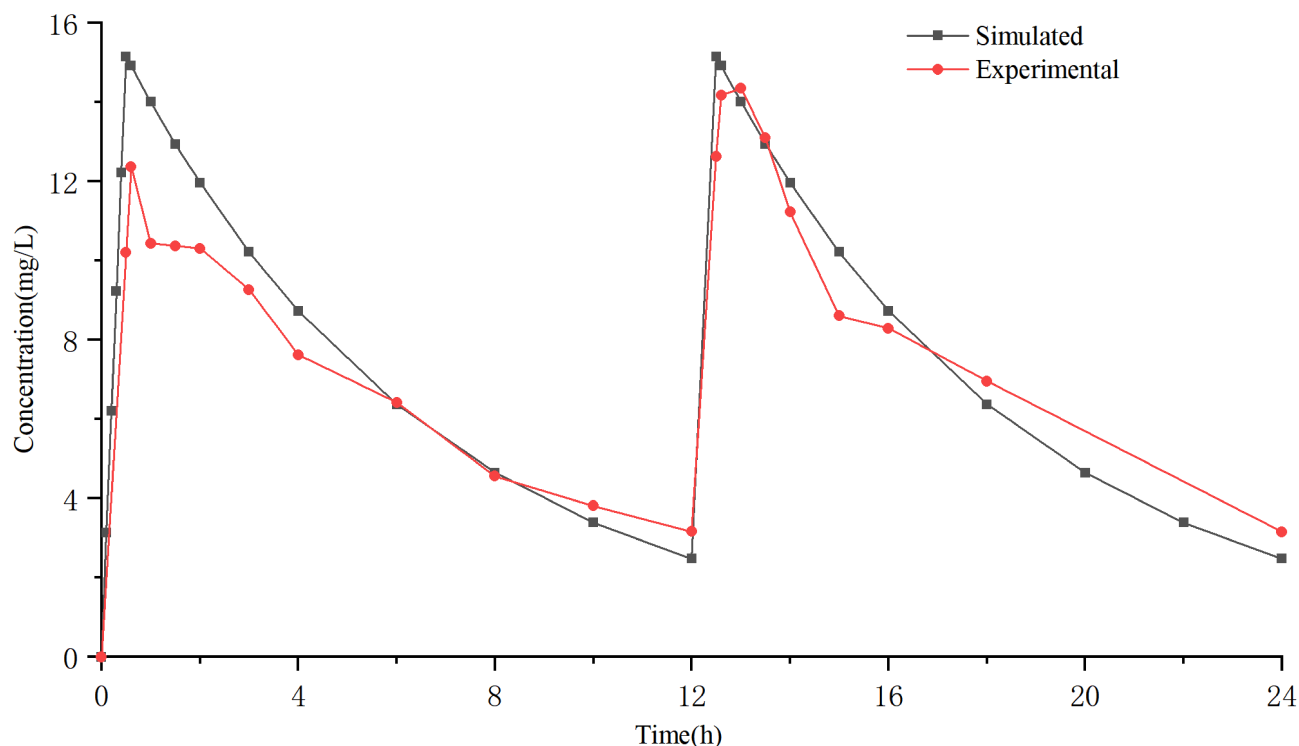
Figure 3 Concentration–time curve.
