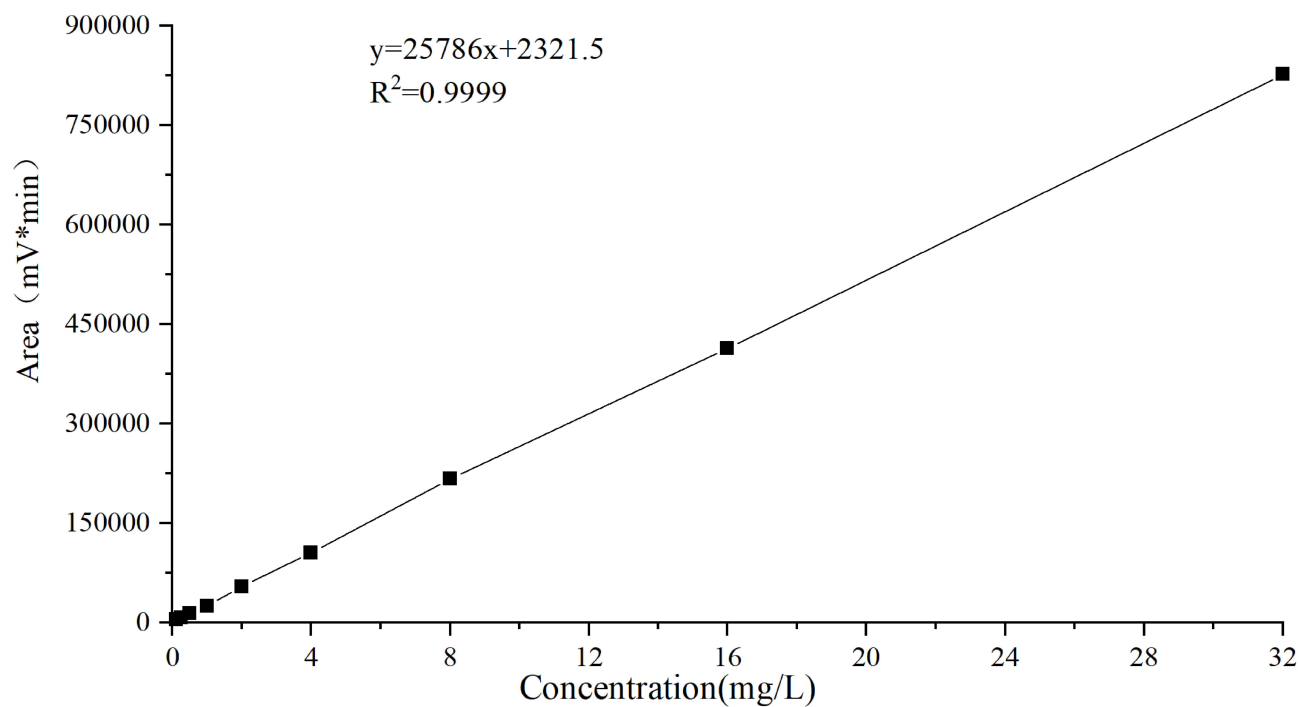
Figure 2 Standard curve.
