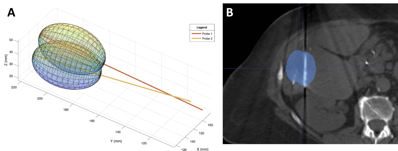
Figure 2 (A) Example case of antenna orientations and predicted Neuwave PR antenna ablation volumes at 65 W for 10 min. Axes represent pixel locations in isotropic volume. Tips are separated by distance of 15.7 mm with 8.30 degrees acute angle between the antennas. Total calculated ablation volume is 34,512 mm 3 . Maximum predicted ablation volume for 2 antennas with 0% overlap is 44,296 mm 3 . As a result, total volumetric overlap of antennas in configuration above is 44.2%. (B) Theoretical modeled ablation zones overlaid on intraprocedural CT scan. Of note, overlapping ablations were predicted to be additive than synergistic.
