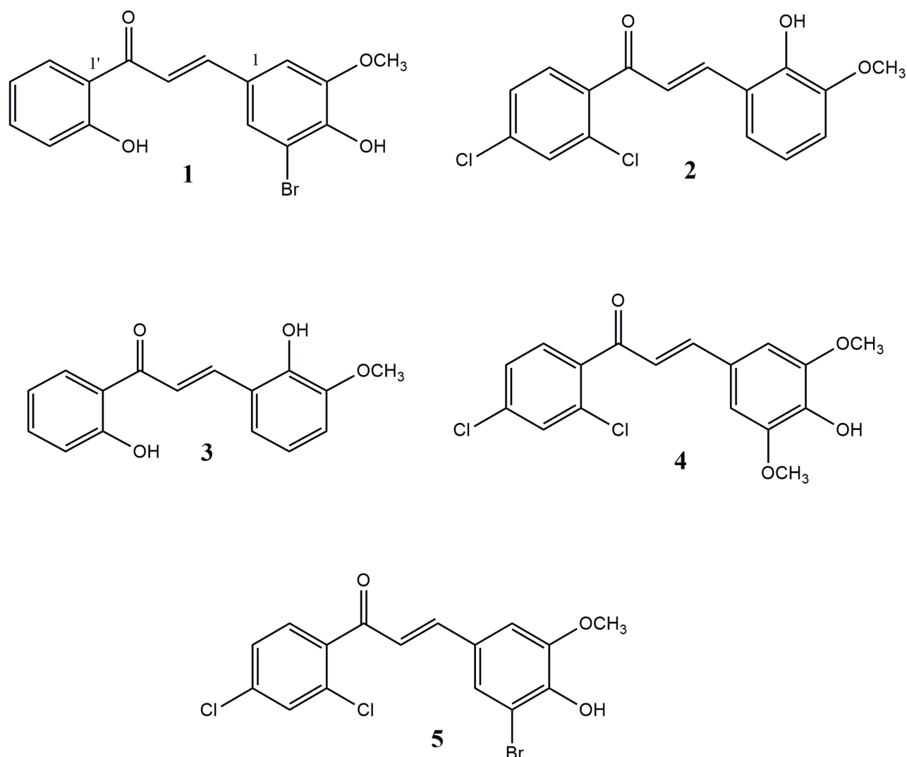
Figure 2 Chemical structure of the synthesized compounds (1–5).
