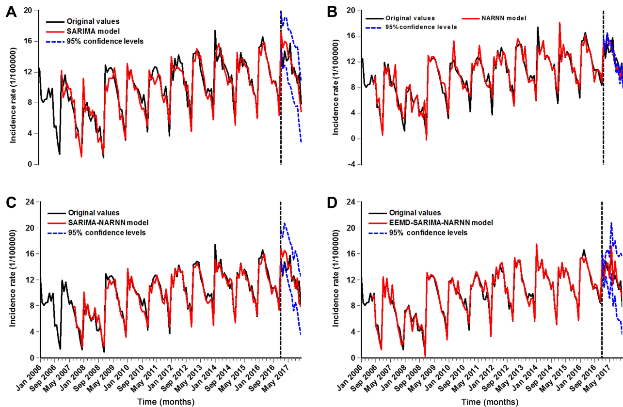
Figure 4 Time series plot showing the comparative results between original observations and fitted and predicted values using the selected best-fitting (A) SARIMA model, (B) NARNN model, (C) traditional SARIMA-NARNN hybrid model, and (D) novel EEMD-SARIMA-NARNN hybrid model (The curve at the left of the vertical black dotted line represents the fitted values, whereas the curve at the right denotes the forecasted values). As shown, the produced curve from the EEMD-SARIMA-NARNN hybrid model is closer to the actual both in the fitted and predicted aspects compared with the curves from the other models.
