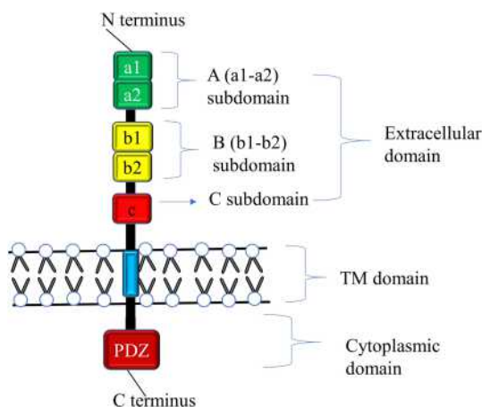
Figure 1 Schematic diagram of NRP1 Structure. NRP1 contains a large N-terminus extracellular domain comprising A (a1-a2), B (b1-b2), and C subdomains, a very small single-pass plasma membrane spanning TM domain, and a short cytoplasmic domain in the inner side of the cell membrane possessing PDZ-binding motif that can interact with various proteins. The a1/a2/b1 segment binds with SEMA3s, VEGFs, and other proteins, and the C domain involved in receptor dimerization with the TM domain. The b1 of NRP1 binds with S protein of SARS-CoV-2 and facilitate infection.
