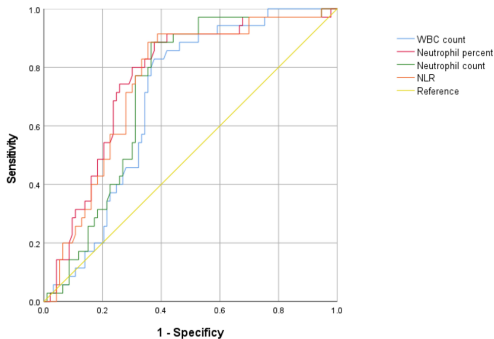
Figure 1 Receiver operating curve of affecting variables to diagnose mature ovarian teratoma with torsion. Combination consists of WBC count, neutrophil percent, neutrophil count, and NLR.
