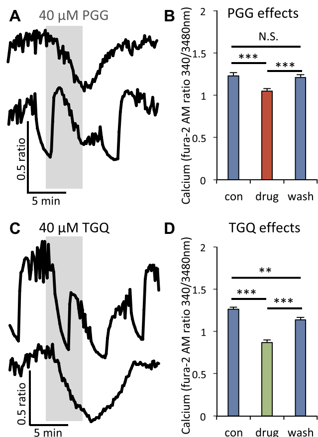
Figure 3 \alpha -PGG and 6Cl-TGQ reduced glucose-stimulated intracellular calcium [ \text{Ca}^{2+} ] i response. (A and C) [ \text{Ca}^{2+} ] i traces showing effects of 5-min exposure to \alpha -PGG (A) and 6Cl-TGQ (C) in 16mM glucose. (B and D) Mean intracellular calcium \pm SEM before (con), during (drug), and after (wash) exposure to \alpha -PGG (B) and 6Cl-TGQ (D). N=10–15 islets were used for testing each compound. N.S. = not significant, ** P < 0.01 , *** P < 0.001 .
