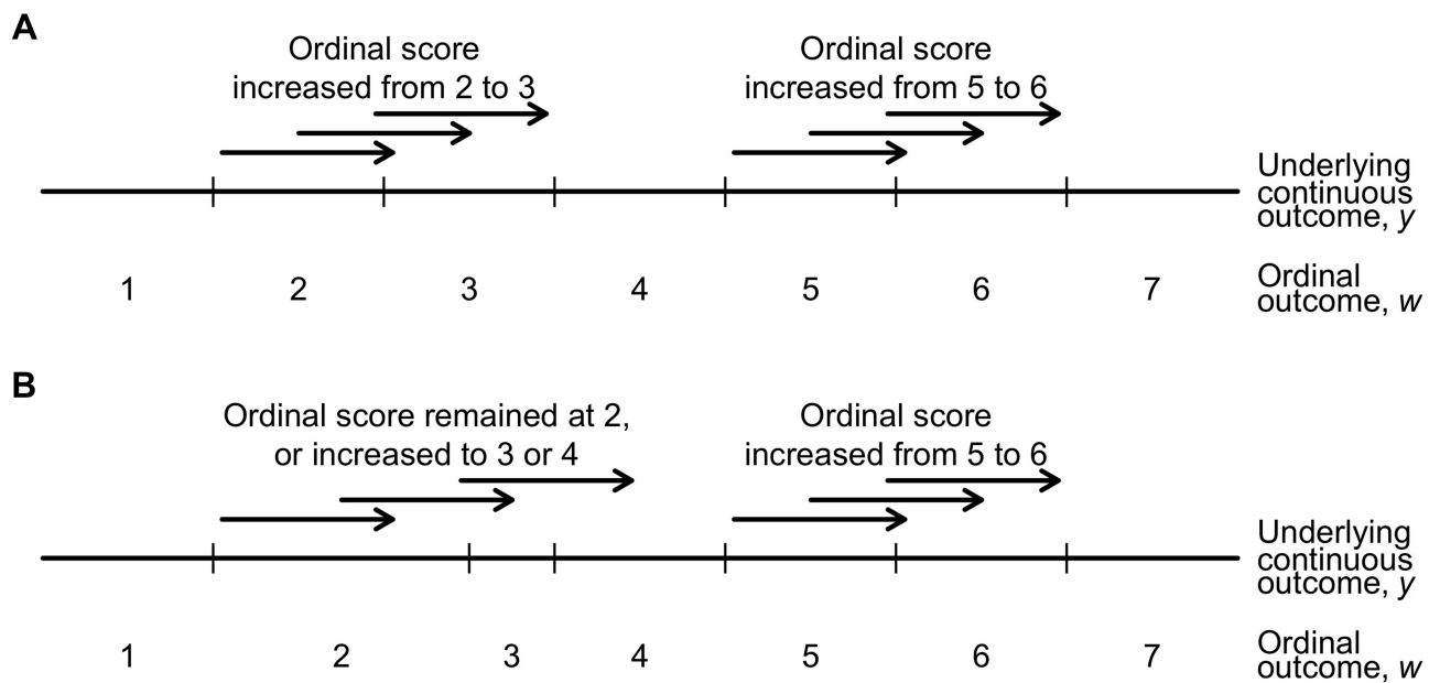
Figure 6 An illustration of a one-unit change (indicated by an arrow pointing to the right) along the continuum of the underlying continuous outcome ( y ) and the corresponding change in the observed ordinal outcome ( w ) when the thresholds (indicated by vertical ticks) are equidistant ( A ) and non-equidistant ( B ).
