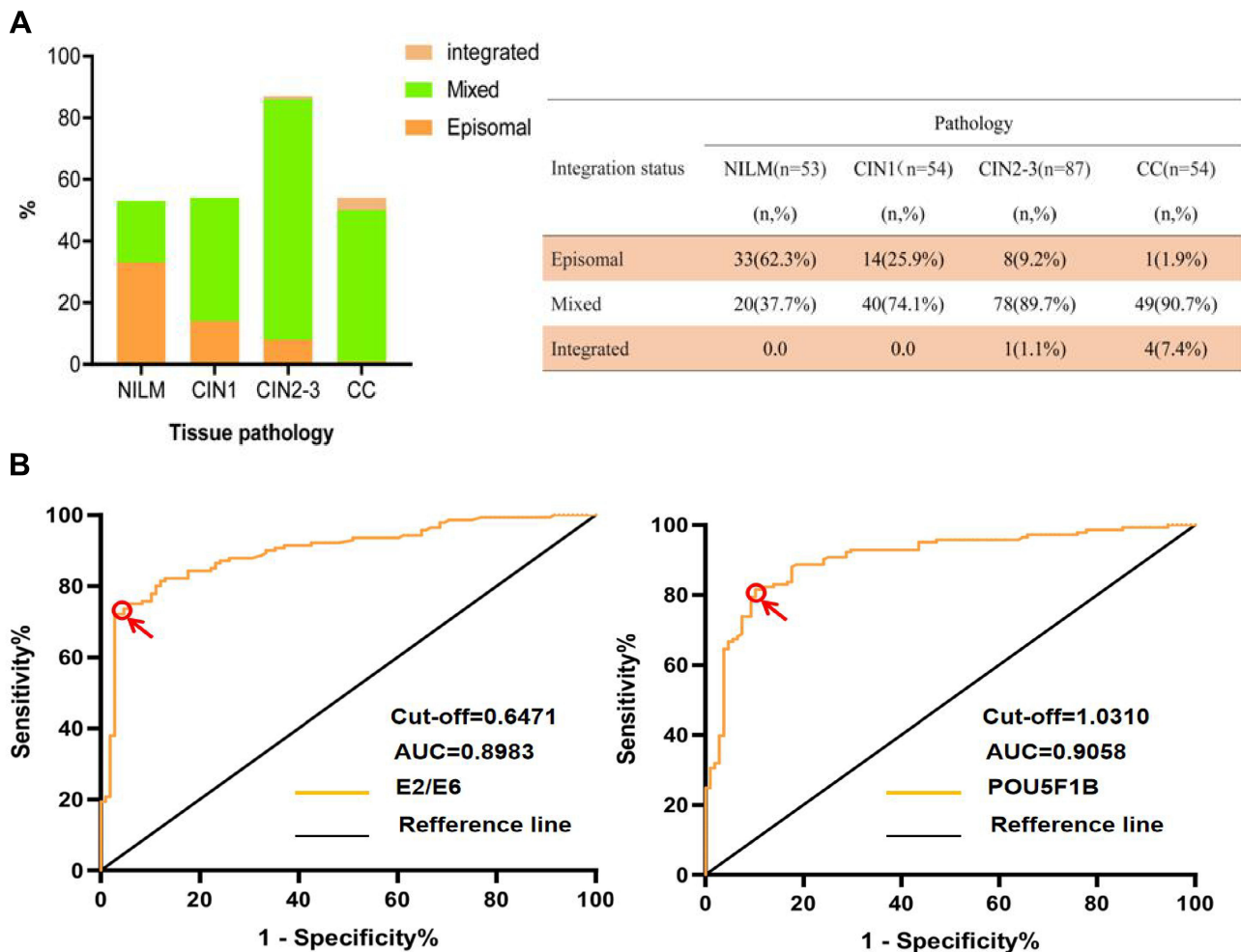
Figure 2 The physical status of HPV infection in HPV16-positive cervical lesions and ROC curve analysis of the HPV-E2/E6 and POU5F1B for identifying CIN2+ disease. (A) The physical status of HPV infection in HPV16-positive cervical lesions (normal, CIN1, CIN2/3, and SCC). A linear association was found between the status of HPV integration and degrees of cervical lesions. (B) Cut-off, the optimal of HPV-E2/E6 and POU5F1B used to predict CIN2+ calculated according to the ROC curve.
