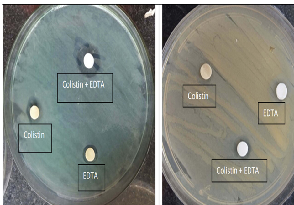
Figure 2 Phenotypic detection for mcr positive isolates by combined disc diffusion test (CDT). (A): mcr-I positive strain showed an increase in the zone diameter of discs with colistin and EDTA \geq 3 mm in comparison to colistin alone. (B): mcr-I negative isolate showed slight change (1 mm) in the inhibition zone diameter of colistin and EDTA disc in comparison to colistin alone.
