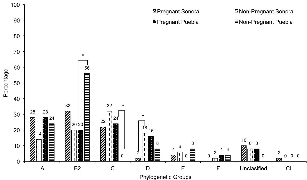
Figure 3 Distribution of phylogenetic group among 150 E. coli strains isolated from urine of women from Sonora and Puebla, Mexico. The statistically significance results ( p < 0.05 ) are in asterisk.
