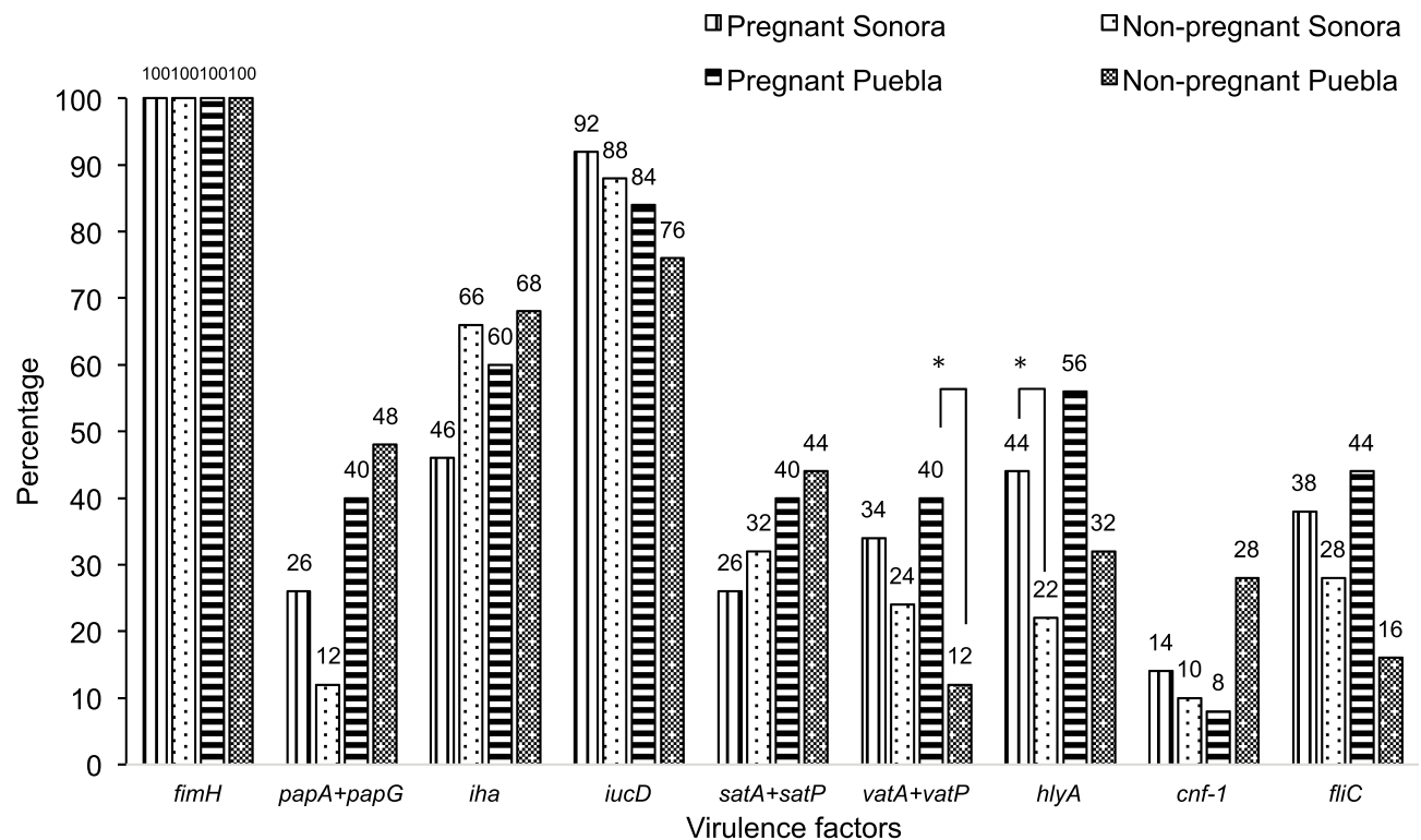
Figure 2 Frequency of the Virulence Genes Among 150 E. coli Isolates From Urine of Pregnant and Non-Pregnant Women From Sonora and Puebla, Mexico. The studied genes encoded the following virulence factor: fimH , type I pilus adhesin; papG+papA , adhesin and pilin of the type P pili; iha , enterobactin receptor/Irg homologue adhesin; iucD , aerobactin; satA+satP , autotransporter and peptidase regions of the secreted autotransporter toxin; vatA+vatP , autotransporter and peptidase regions of the vacuolating autotransporter toxin; hlyA , \alpha -hemolysin; cnf-1 , cytotoxic necrotizing factor; fliC , flagellin. The statistically significance results ( p < 0.05 ) are in asterisk.
