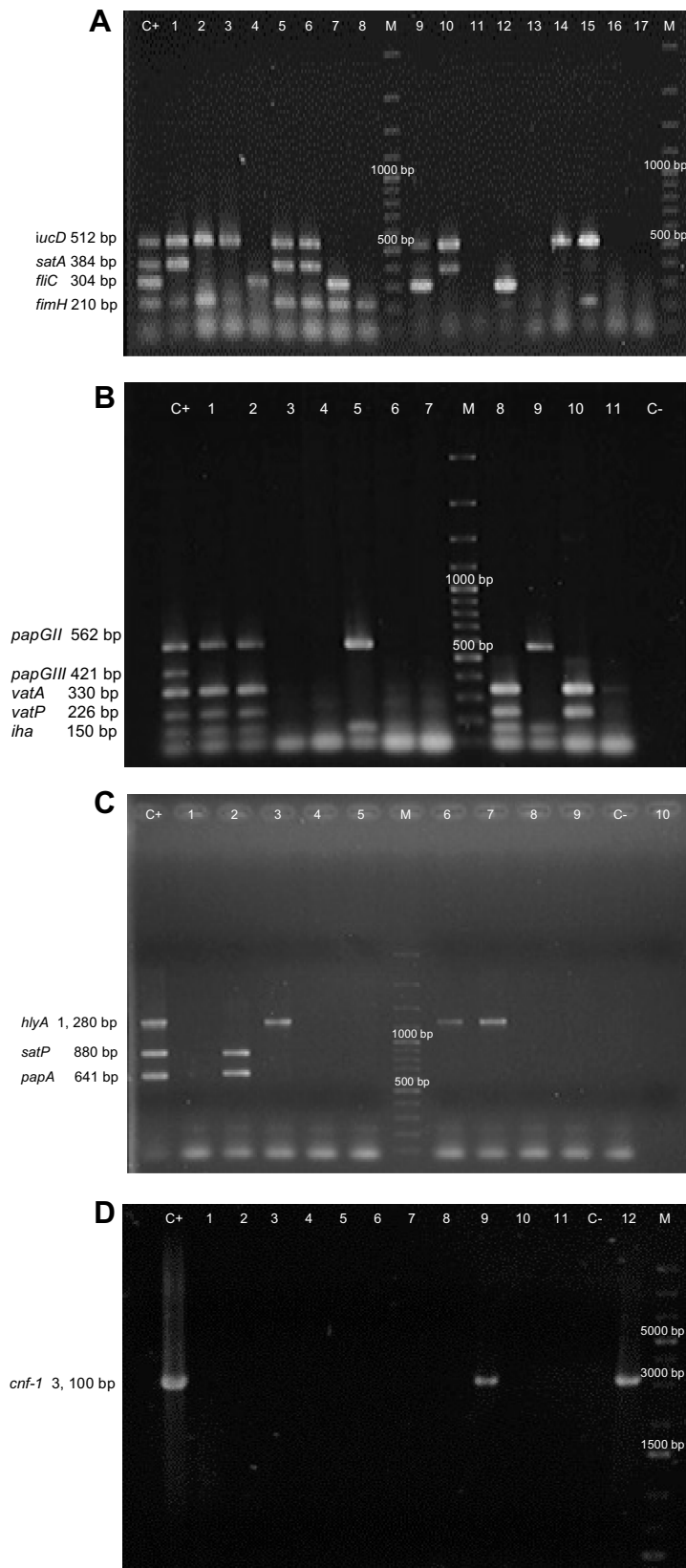
Figure 1 Multiplex-PCR Banding Patterns of Virulence Genes and Individual PCRCnf of E. coli generated by gel electrophoresis. (A) iucD (512 bp), satA (384 bp) and fimH (210 bp). (B) papGII (562 bp), papGIII (421 bp); vatA (330 bp), vatP (226 bp) and iha (150bp). (C) hlyA (1,280 bp), satP (880 bp) and papA (641 bp). (D) cnf-1 (3,100 bp). M. Molecular weight market (100 bp Plus DNA Ladder in A , B and C and 1 kb Plus DNA ladder in D ) . Lane C+. Positive control ( E. coli CFTO73 in A ; E. coli CFTO73 plus E. coli O59I in B and E. coli GAGI in C and D ) . Lines with a number E. coli isolated from the samples. C-. Negative control.
