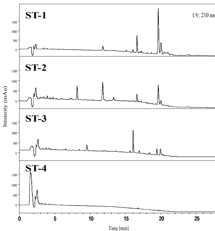
Figure 1 HPLC-DAD chromatograms of S-T 1 – ST-4. HPLC stationary phase: Phenomenex Synergi Polar RP column (150 \times 4.6 mm, 4 \mu\text{m} ); mobile phase: water (A) and acetonitrile (B) (both with 0.1% acetic acid), gradient: 65% A to 50% A in 10 min, from 50% to 2% in 10 min; flow rate: 1 ml/min; temperature: 25 ^{\circ}\text{C} ; injection volume: 10 \mu\text{l} .
